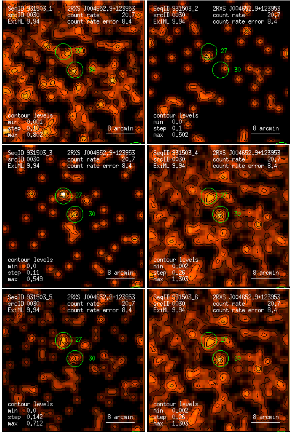
Figure 30: RASS 931503: detection 0030: band rate images, Gaussian filter: (1) PSPC channels 11 – 41, (2) 52 – 90, (3) 91 – 201, (4) 11 – 235, (5) 52 – 201, (6) 11 – 201. Broad band rates in counts/ks. Band rate contour levels in counts/ks/arcmin 2 .
