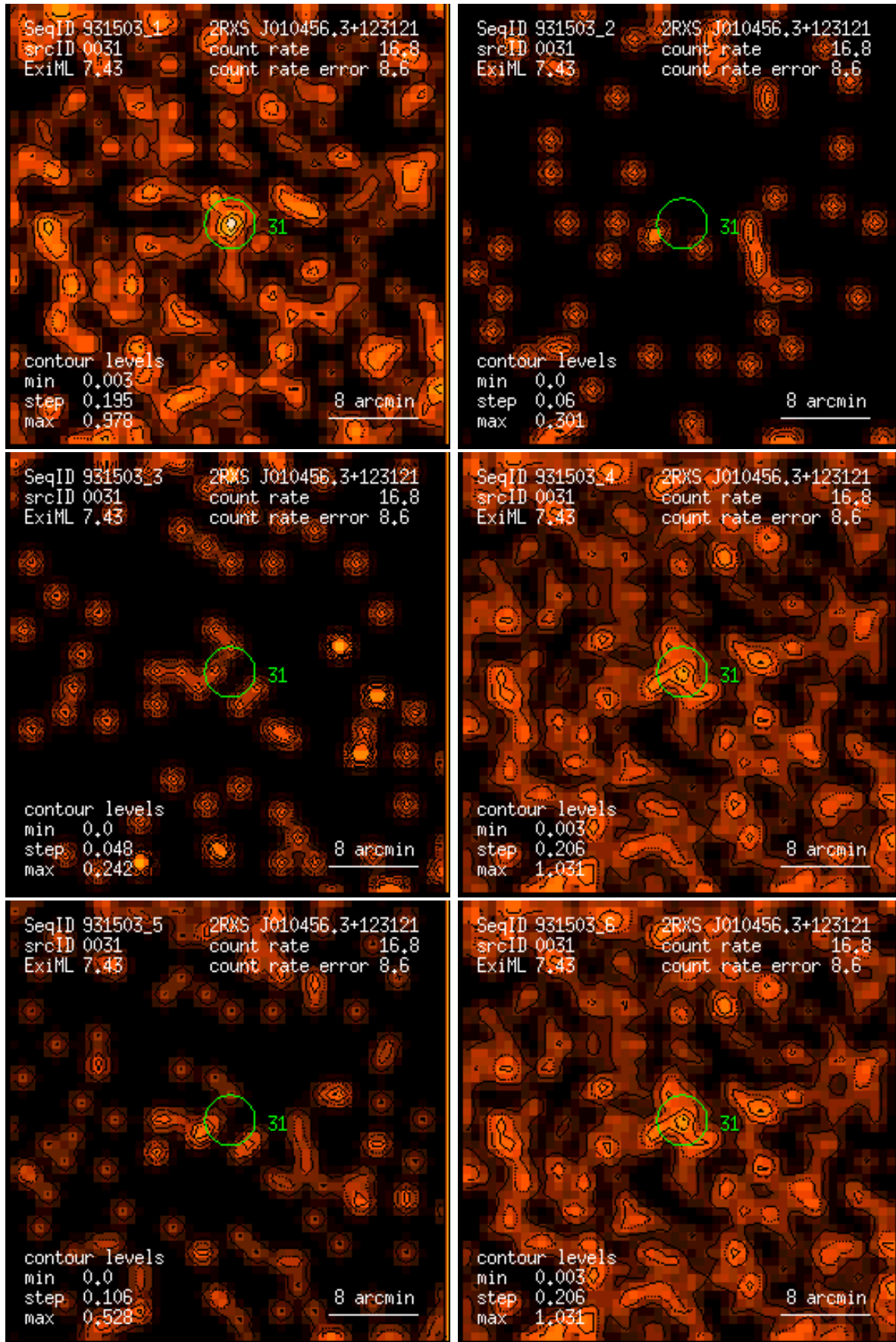
Figure 31: RASS 931503: detection 0031: band rate images, Gaussian filter: (1) PSPC channels 11 – 41, (2) 52 – 90, (3) 91 – 201, (4) 11 – 235, (5) 52 – 201, (6) 11 – 201. Broad band rates in counts/ks. Band rate contour levels in counts/ks/arcmin 2 .
