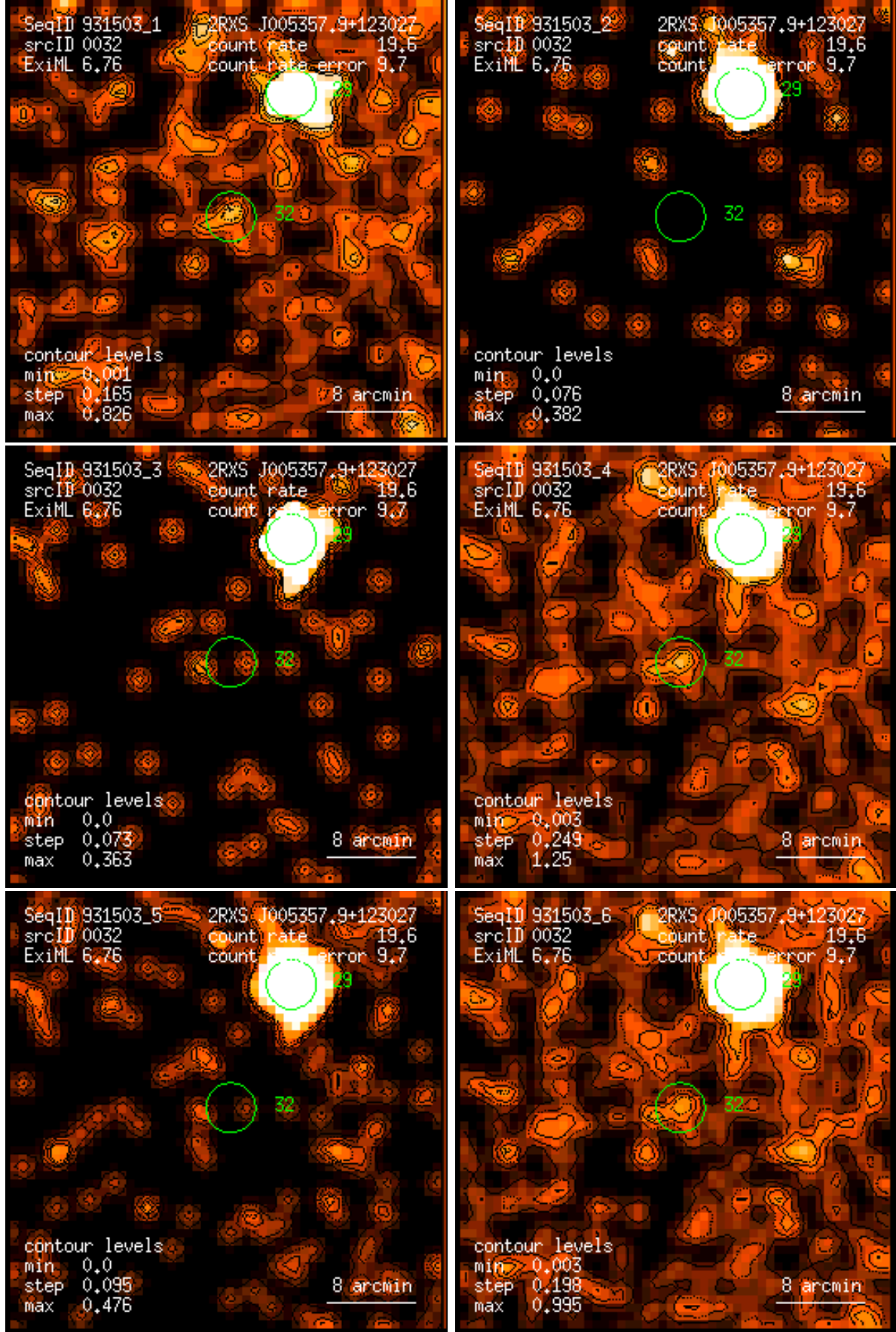
Figure 32: RASS 931503: detection 0032: band rate images, Gaussian filter: (1) PSPC channels 11 – 41, (2) 52 – 90, (3) 91 – 201, (4) 11 – 235, (5) 52 – 201, (6) 11 – 201. Broad band rates in counts/ks. Band rate contour levels in counts/ks/arcmin 2 .
