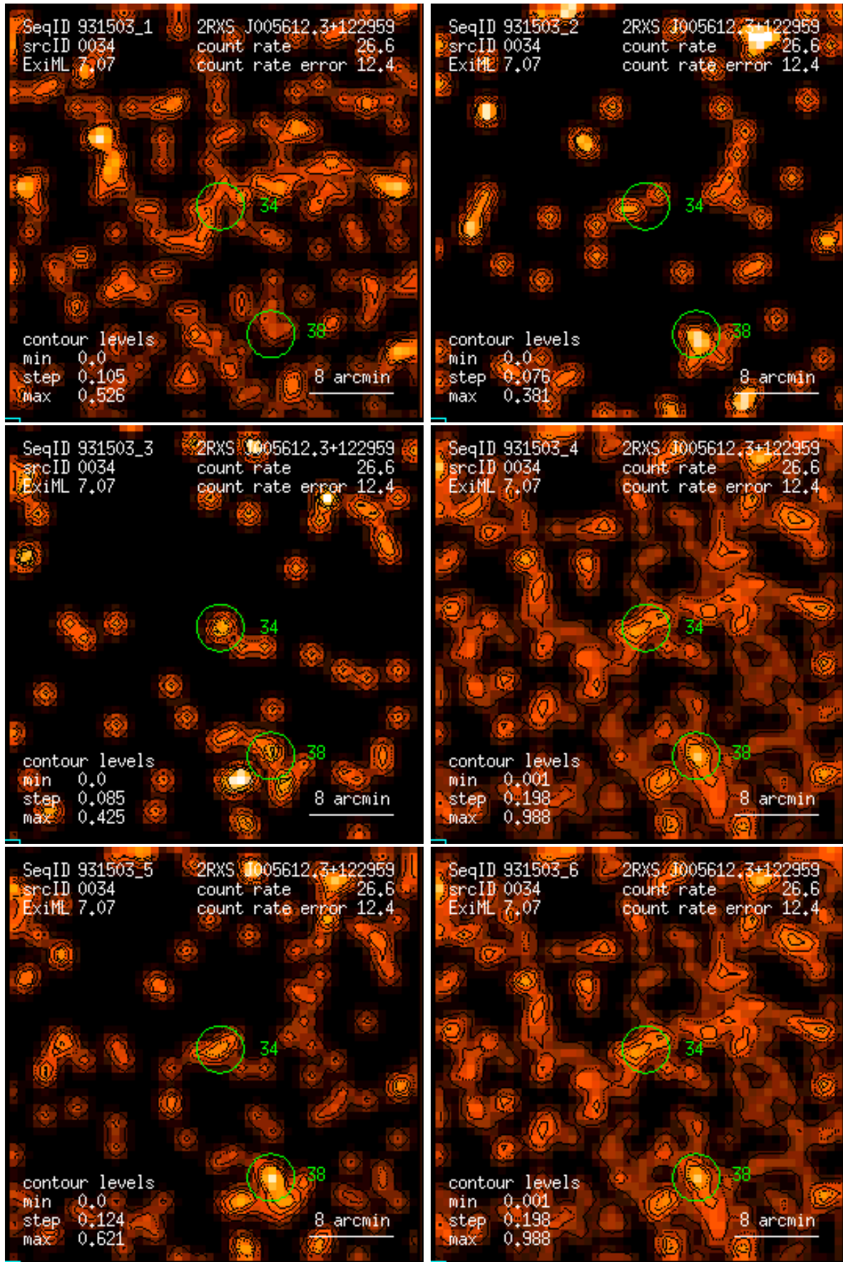
Figure 34: RASS 931503: detection 0034: band rate images, Gaussian filter: (1) PSPC channels 11 – 41, (2) 52 – 90, (3) 91 – 201, (4) 11 – 235, (5) 52 – 201, (6) 11 – 201. Broad band rates in counts/ks. Band rate contour levels in counts/ks/arcmin 2 .
