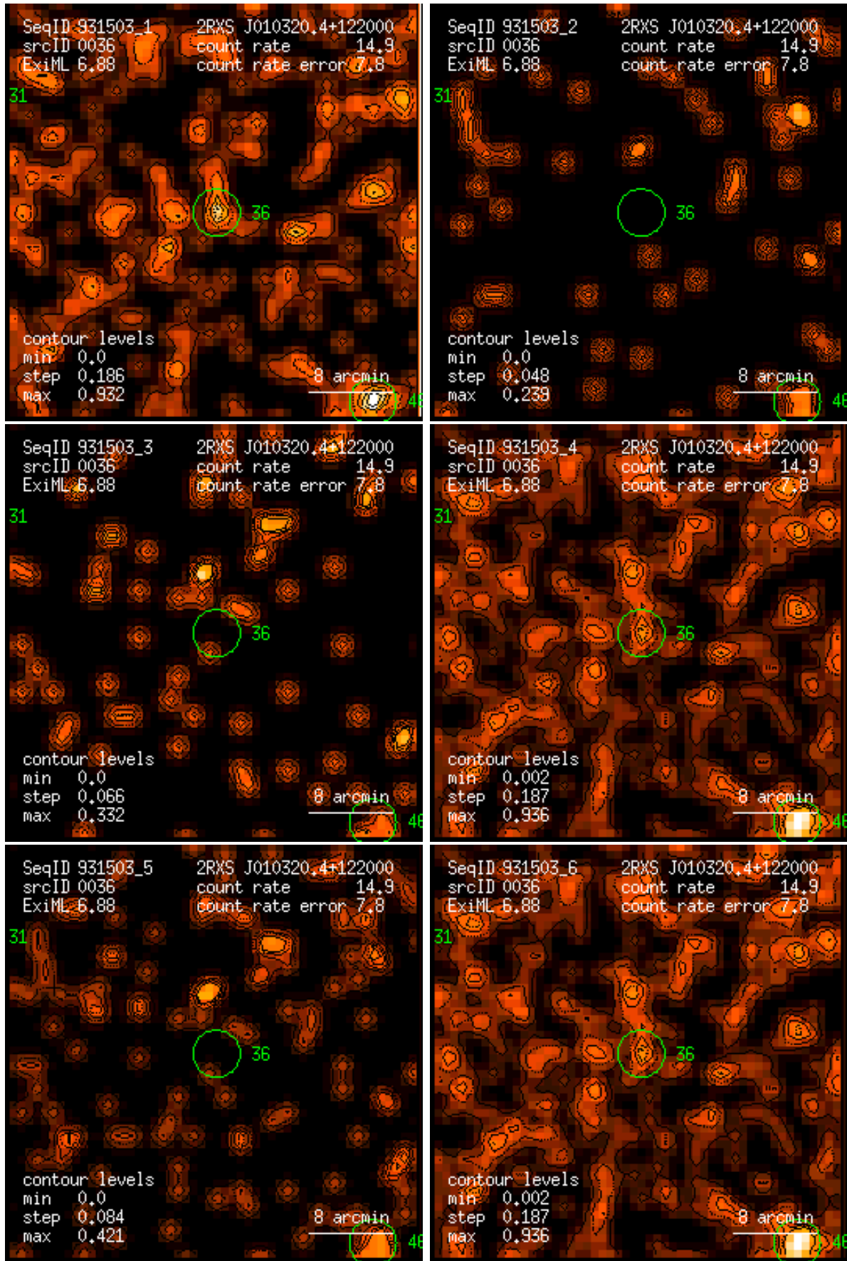
Figure 36: RASS 931503: detection 0036: band rate images, Gaussian filter: (1) PSPC channels 11 – 41, (2) 52 – 90, (3) 91 – 201, (4) 11 – 235, (5) 52 – 201, (6) 11 – 201. Broad band rates in counts/ks. Band rate contour levels in counts/ks/arcmin 2 .
