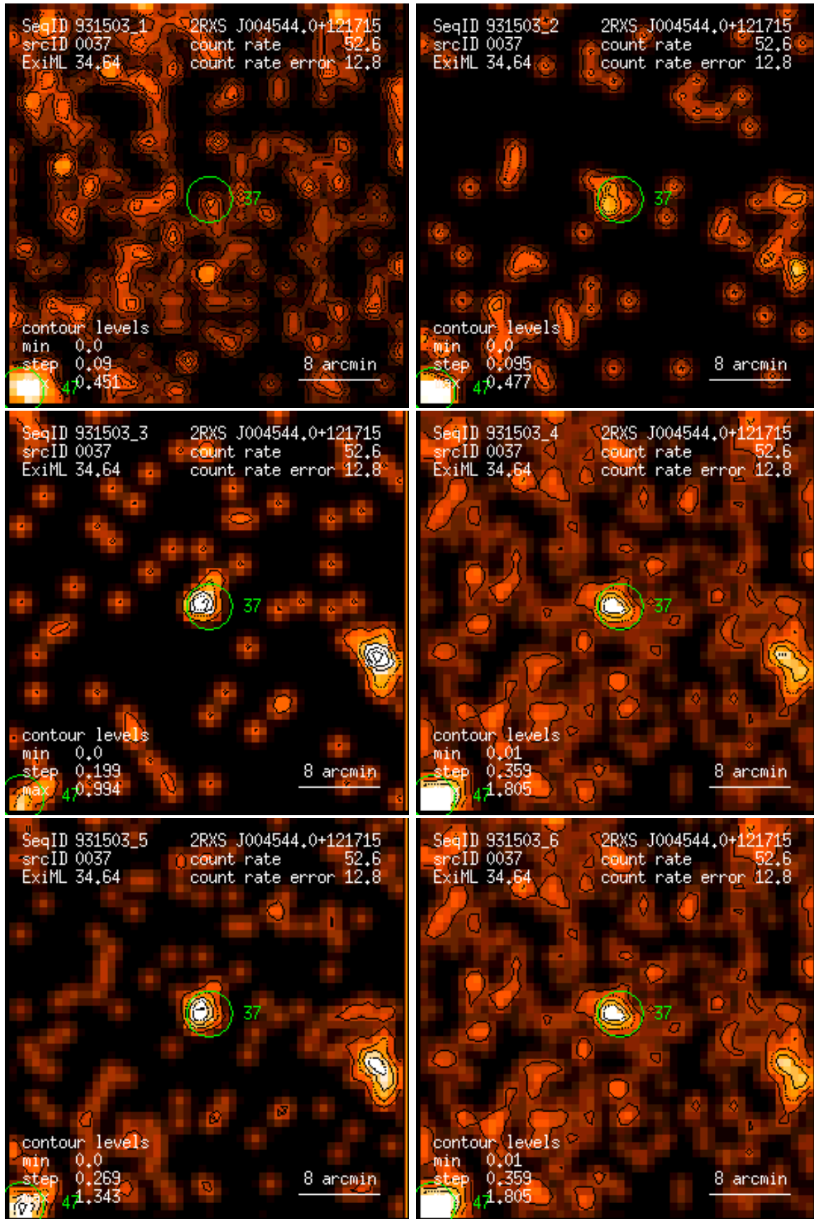
Figure 37: RASS 931503: detection 0037: band rate images, Gaussian filter: (1) PSPC channels 11 – 41, (2) 52 – 90, (3) 91 – 201, (4) 11 – 235, (5) 52 – 201, (6) 11 – 201. Broad band rates in counts/ks. Band rate contour levels in counts/ks/arcmin 2 .
