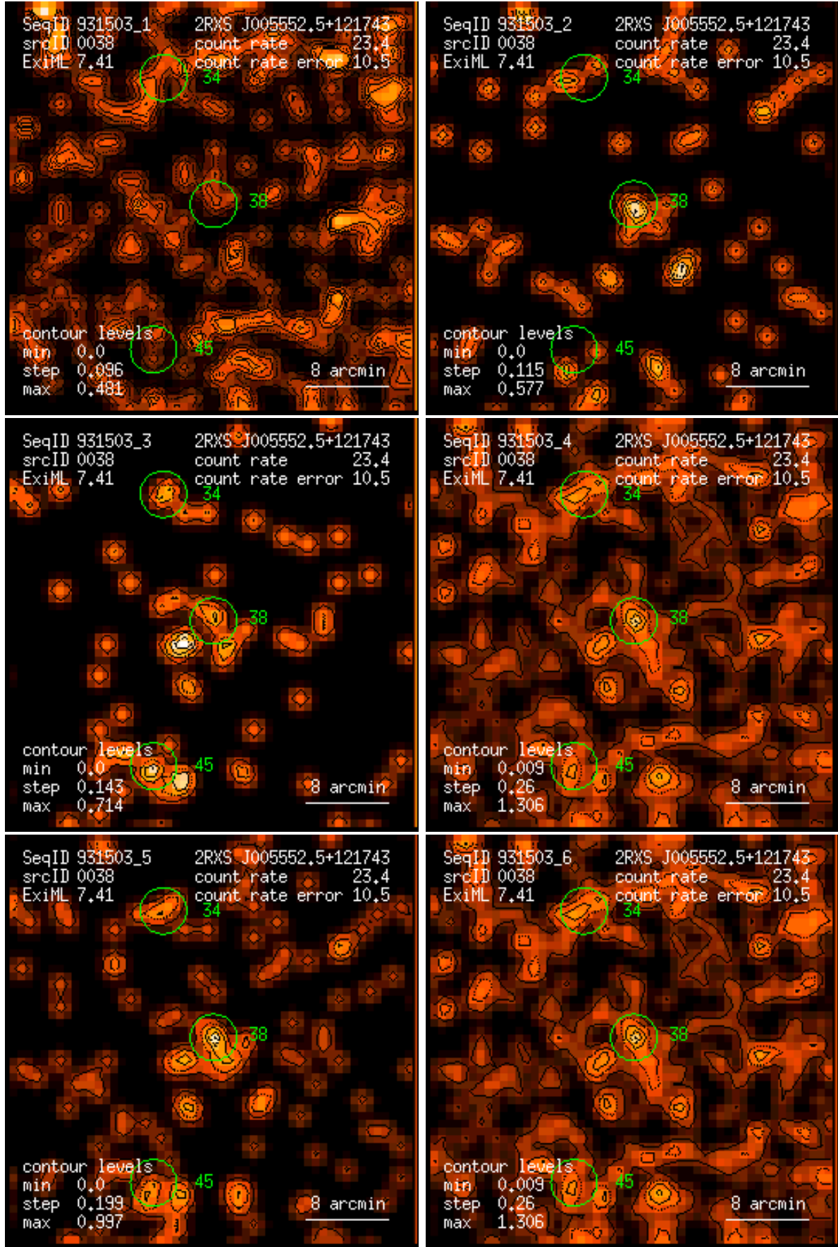
Figure 38: RASS 931503: detection 0038: band rate images, Gaussian filter: (1) PSPC channels 11 – 41, (2) 52 – 90, (3) 91 – 201, (4) 11 – 235, (5) 52 – 201, (6) 11 – 201. Broad band rates in counts/ks. Band rate contour levels in counts/ks/arcmin 2 .
