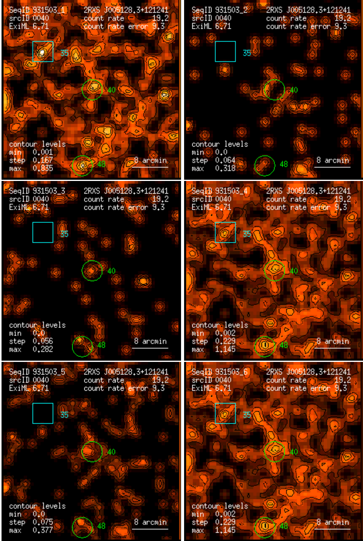
Figure 40: RASS 931503: detection 0040: band rate images, Gaussian filter: (1) PSPC channels 11 – 41, (2) 52 – 90, (3) 91 – 201, (4) 11 – 235, (5) 52 – 201, (6) 11 – 201. Broad band rates in counts/ks. Band rate contour levels in counts/ks/arcmin 2 .
