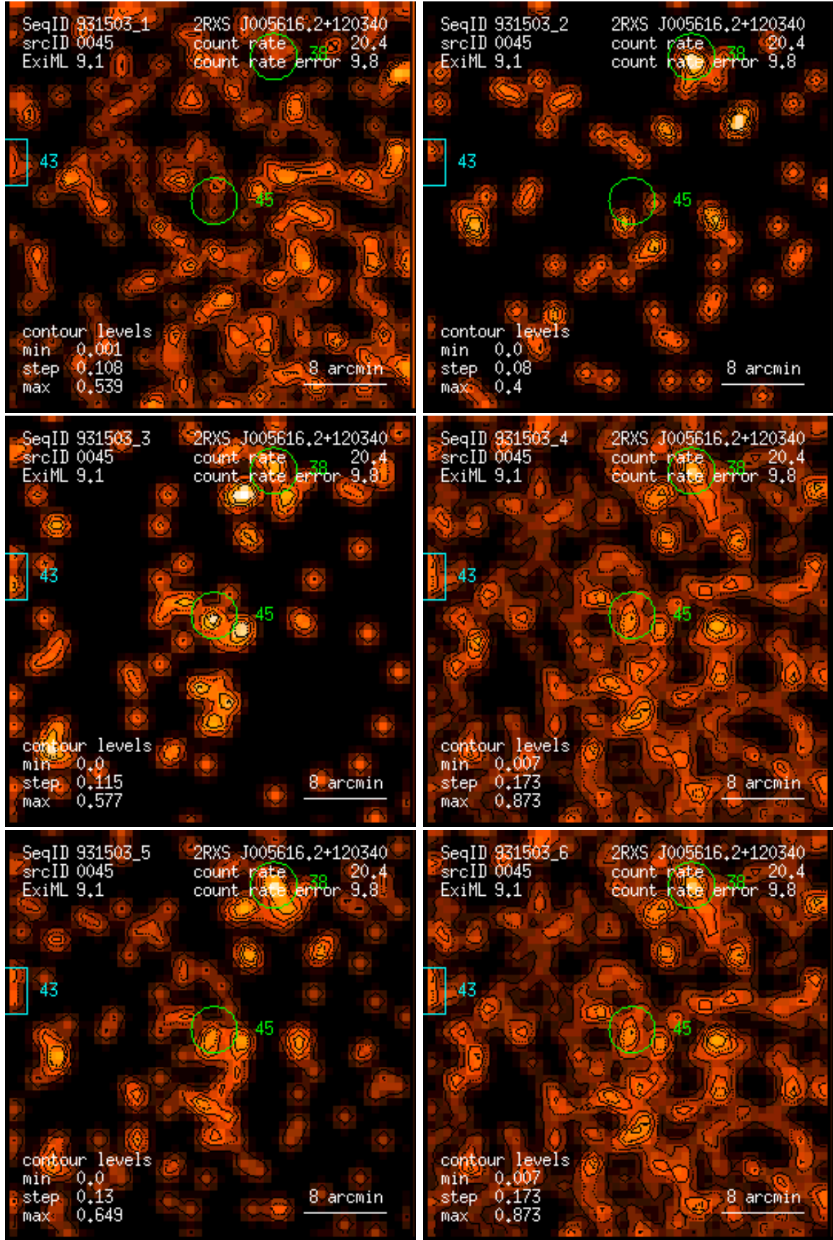
Figure 45: RASS 931503: detection 0045: band rate images, Gaussian filter: (1) PSPC channels 11 – 41, (2) 52 – 90, (3) 91 – 201, (4) 11 – 235, (5) 52 – 201, (6) 11 – 201. Broad band rates in counts/ks. Band rate contour levels in counts/ks/arcmin 2 .
