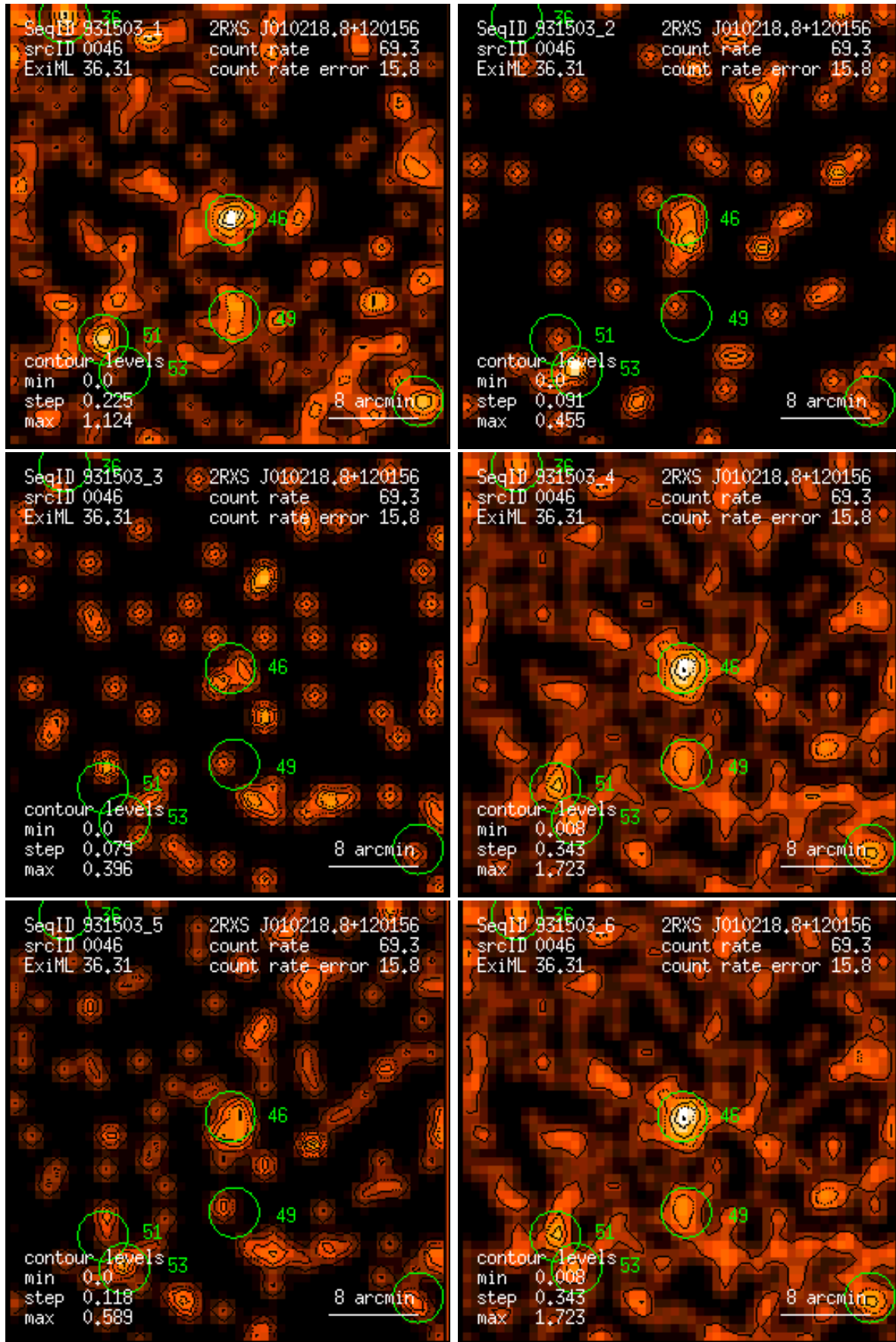
Figure 46: RASS 931503: detection 0046: band rate images, Gaussian filter: (1) PSPC channels 11 – 41, (2) 52 – 90, (3) 91 – 201, (4) 11 – 235, (5) 52 – 201, (6) 11 – 201. Broad band rates in counts/ks. Band rate contour levels in counts/ks/arcmin 2 .
