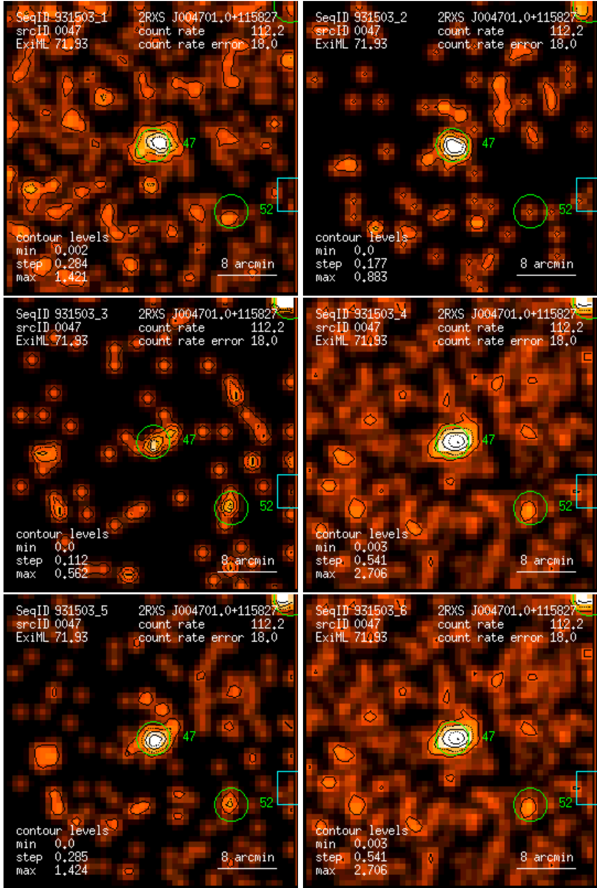
Figure 47: RASS 931503: detection 0047: band rate images, Gaussian filter: (1) PSPC channels 11 – 41, (2) 52 – 90, (3) 91 – 201, (4) 11 – 235, (5) 52 – 201, (6) 11 – 201. Broad band rates in counts/ks. Band rate contour levels in counts/ks/arcmin 2 .
