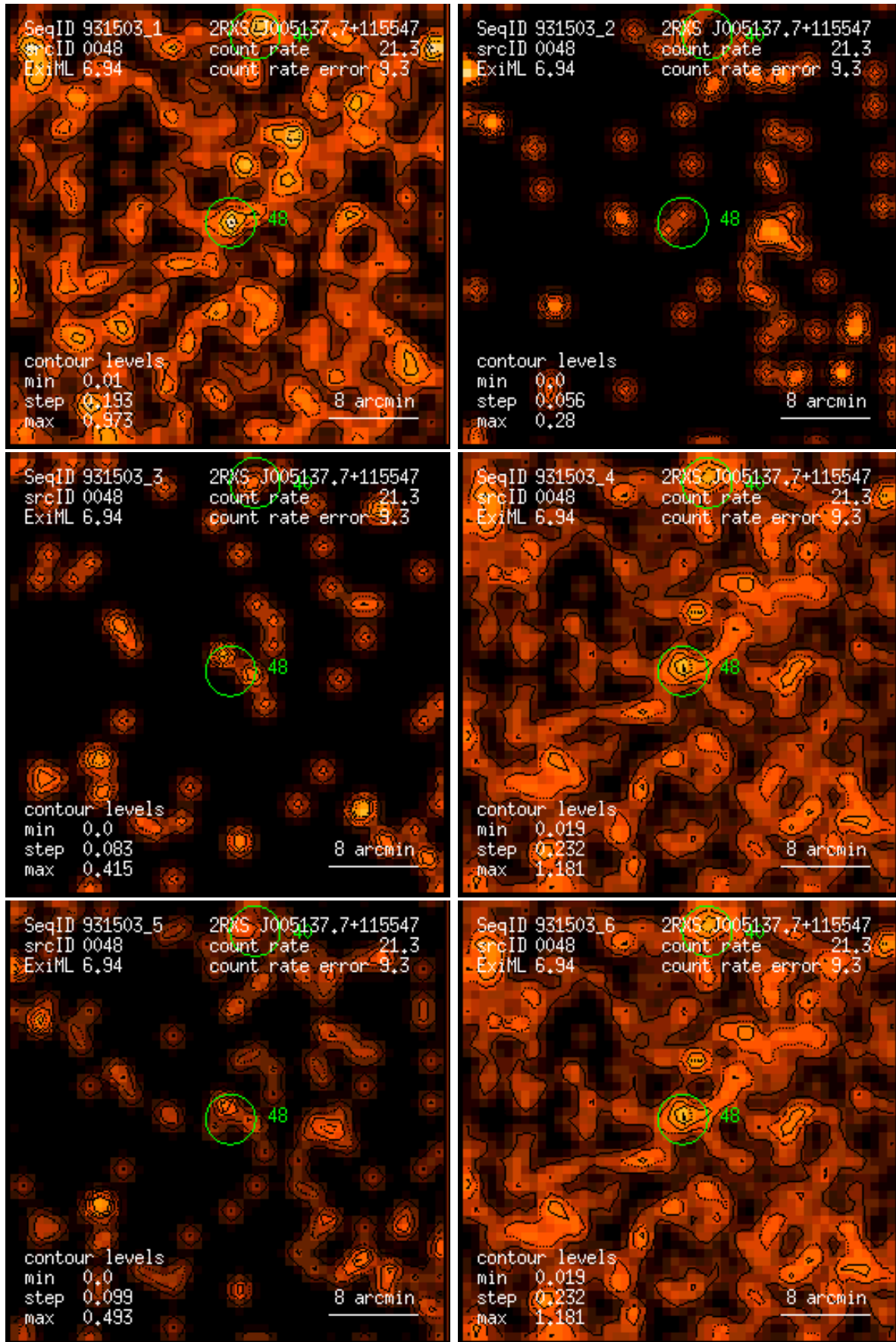
Figure 48: RASS 931503: detection 0048: band rate images, Gaussian filter: (1) PSPC channels 11 – 41, (2) 52 – 90, (3) 91 – 201, (4) 11 – 235, (5) 52 – 201, (6) 11 – 201. Broad band rates in counts/ks. Band rate contour levels in counts/ks/arcmin 2 .
