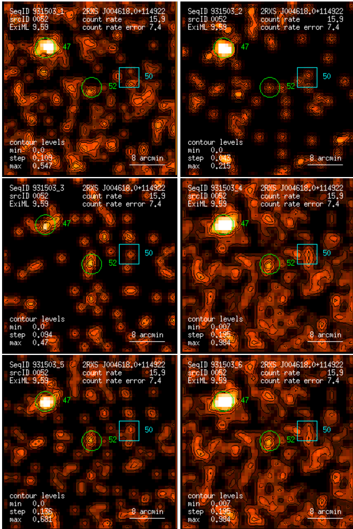
Figure 52: RASS 931503: detection 0052: band rate images, Gaussian filter: (1) PSPC channels 11 – 41, (2) 52 – 90, (3) 91 – 201, (4) 11 – 235, (5) 52 – 201, (6) 11 – 201. Broad band rates in counts/ks. Band rate contour levels in counts/ks/arcmin 2 .
