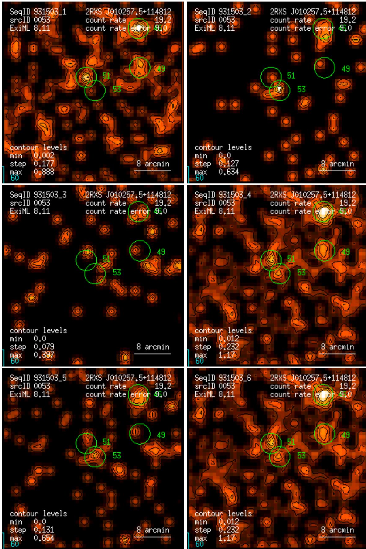
Figure 53: RASS 931503: detection 0053: band rate images, Gaussian filter: (1) PSPC channels 11 – 41, (2) 52 – 90, (3) 91 – 201, (4) 11 – 235, (5) 52 – 201, (6) 11 – 201. Broad band rates in counts/ks. Band rate contour levels in counts/ks/arcmin 2 .
