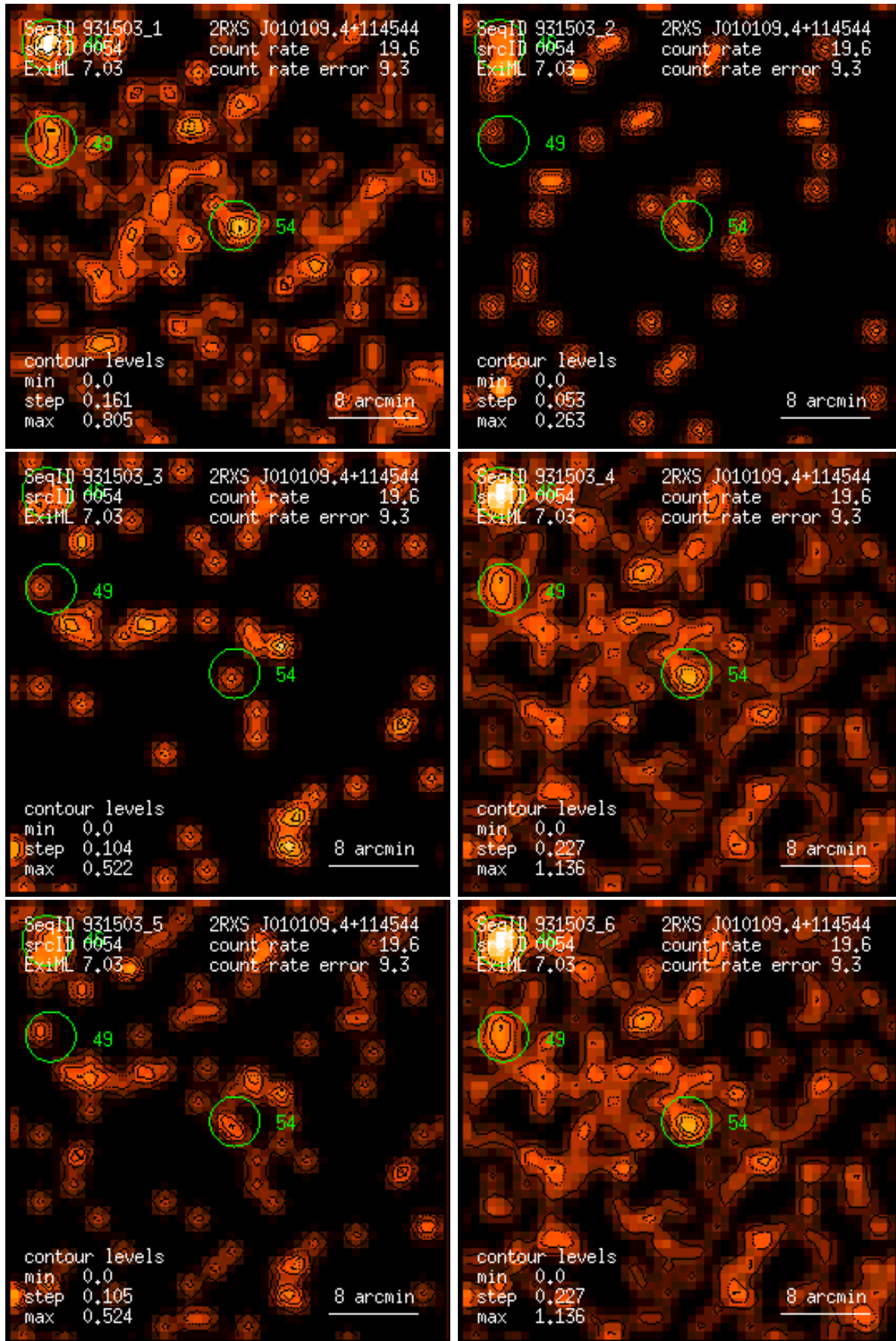
Figure 54: RASS 931503: detection 0054: band rate images, Gaussian filter: (1) PSPC channels 11 – 41, (2) 52 – 90, (3) 91 – 201, (4) 11 – 235, (5) 52 – 201, (6) 11 – 201. Broad band rates in counts/ks. Band rate contour levels in counts/ks/arcmin 2 .
