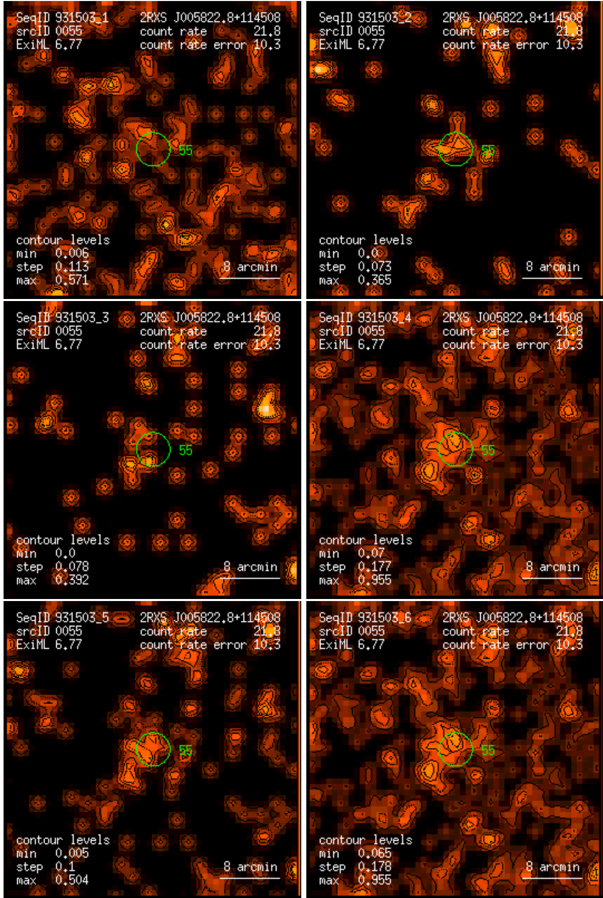
Figure 55: RASS 931503: detection 0055: band rate images, Gaussian filter: (1) PSPC channels 11 – 41, (2) 52 – 90, (3) 91 – 201, (4) 11 – 235, (5) 52 – 201, (6) 11 – 201. Broad band rates in counts/ks. Band rate contour levels in counts/ks/arcmin 2 .
