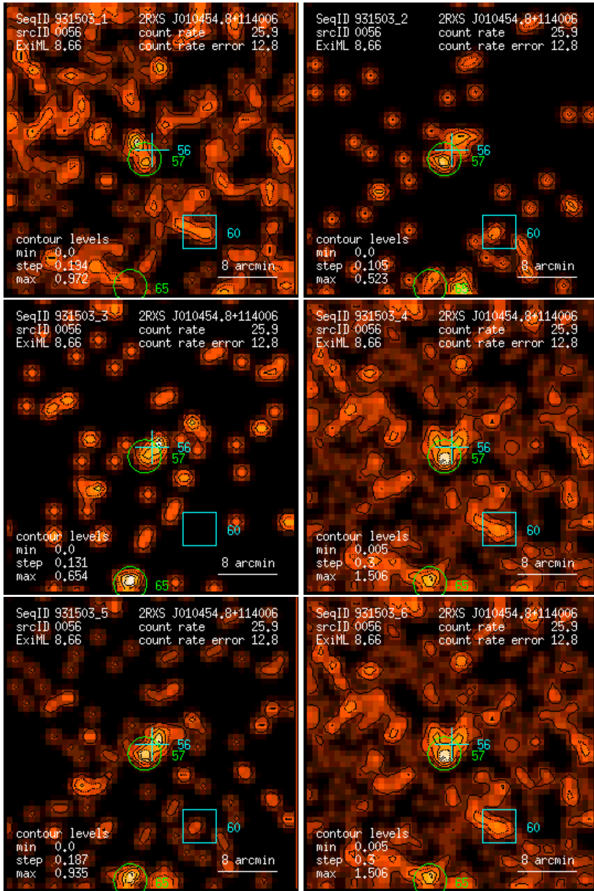
Figure 56: RASS 931503: detection 0056: band rate images, Gaussian filter: (1) PSPC channels 11 – 41, (2) 52 – 90, (3) 91 – 201, (4) 11 – 235, (5) 52 – 201, (6) 11 – 201. Broad band rates in counts/ks. Band rate contour levels in counts/ks/arcmin 2 .
