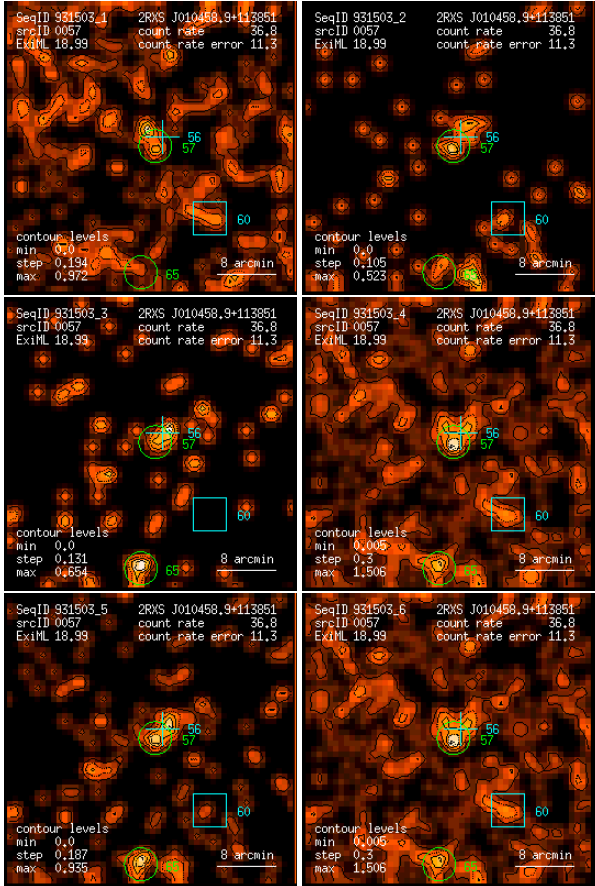
Figure 57: RASS 931503: detection 0057: band rate images, Gaussian filter: (1) PSPC channels 11 – 41, (2) 52 – 90, (3) 91 – 201, (4) 11 – 235, (5) 52 – 201, (6) 11 – 201. Broad band rates in counts/ks. Band rate contour levels in counts/ks/arcmin 2 .
