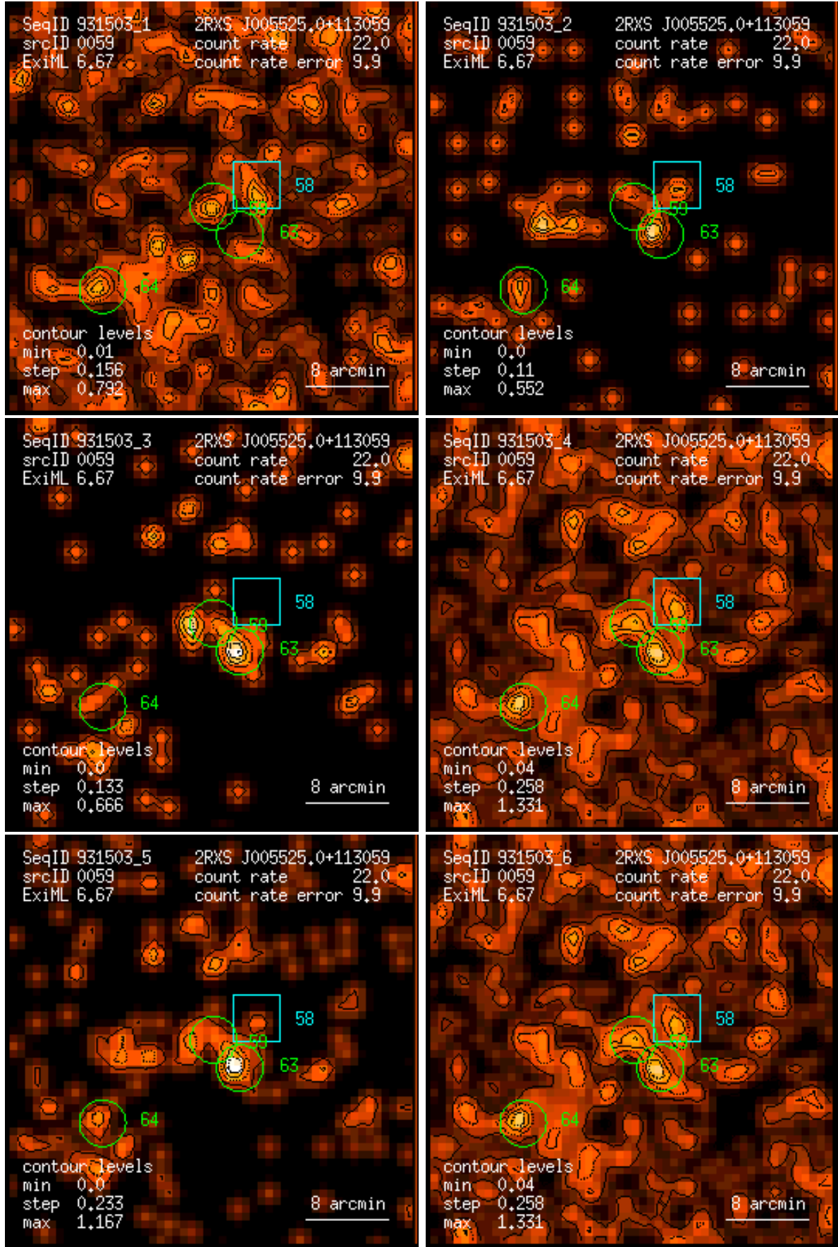
Figure 59: RASS 931503: detection 0059: band rate images, Gaussian filter: (1) PSPC channels 11 – 41, (2) 52 – 90, (3) 91 – 201, (4) 11 – 235, (5) 52 – 201, (6) 11 – 201. Broad band rates in counts/ks. Band rate contour levels in counts/ks/arcmin 2 .
