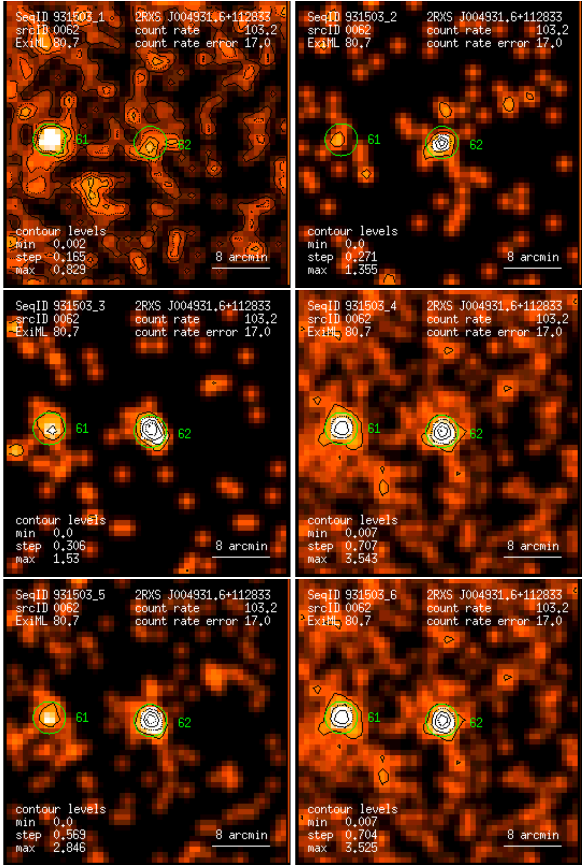
Figure 62: RASS 931503: detection 0062: band rate images, Gaussian filter: (1) PSPC channels 11 – 41, (2) 52 – 90, (3) 91 – 201, (4) 11 – 235, (5) 52 – 201, (6) 11 – 201. Broad band rates in counts/ks. Band rate contour levels in counts/ks/arcmin 2 .
