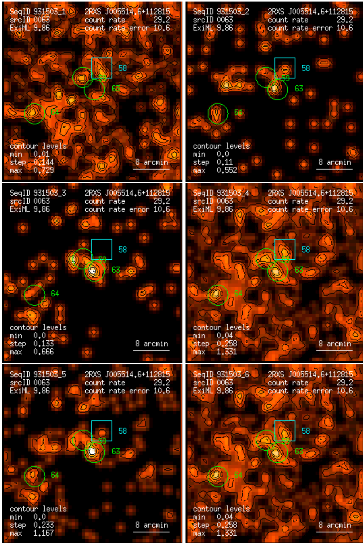
Figure 63: RASS 931503: detection 0063: band rate images, Gaussian filter: (1) PSPC channels 11 – 41, (2) 52 – 90, (3) 91 – 201, (4) 11 – 235, (5) 52 – 201, (6) 11 – 201. Broad band rates in counts/ks. Band rate contour levels in counts/ks/arcmin 2 .
