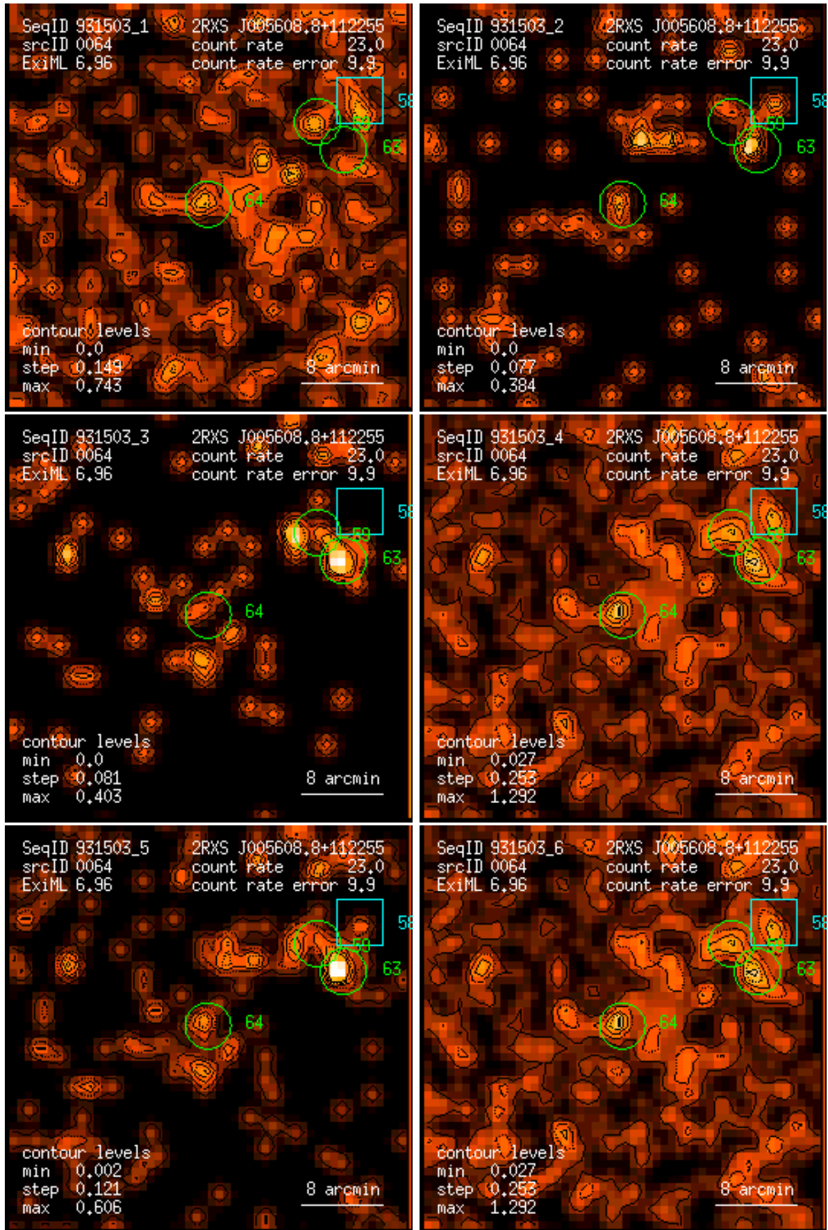
Figure 64: RASS 931503: detection 0064: band rate images, Gaussian filter: (1) PSPC channels 11 – 41, (2) 52 – 90, (3) 91 – 201, (4) 11 – 235, (5) 52 – 201, (6) 11 – 201. Broad band rates in counts/ks. Band rate contour levels in counts/ks/arcmin 2 .
