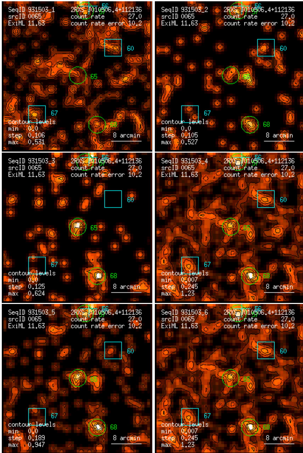
Figure 65: RASS 931503: detection 0065: band rate images, Gaussian filter: (1) PSPC channels 11 – 41, (2) 52 – 90, (3) 91 – 201, (4) 11 – 235, (5) 52 – 201, (6) 11 – 201. Broad band rates in counts/ks. Band rate contour levels in counts/ks/arcmin 2 .
