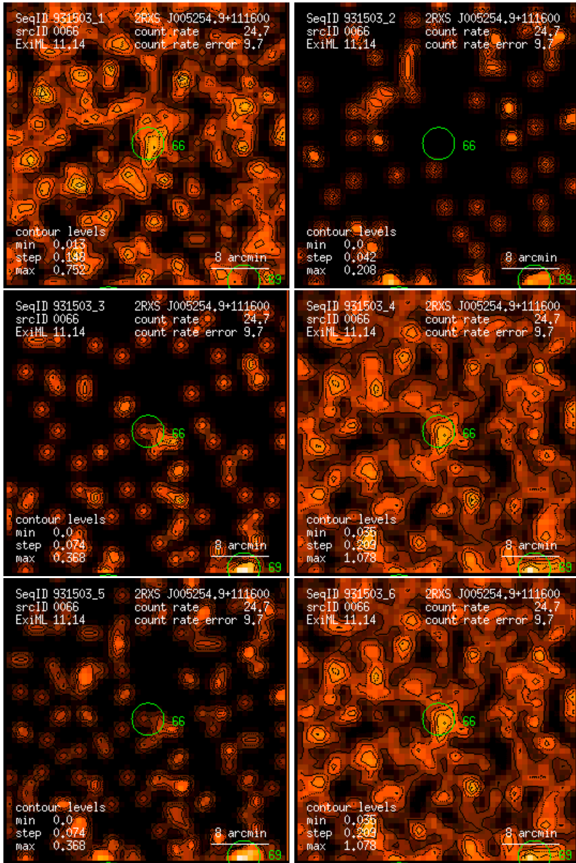
Figure 66: RASS 931503: detection 0066: band rate images, Gaussian filter: (1) PSPC channels 11 – 41, (2) 52 – 90, (3) 91 – 201, (4) 11 – 235, (5) 52 – 201, (6) 11 – 201. Broad band rates in counts/ks. Band rate contour levels in counts/ks/arcmin 2 .
