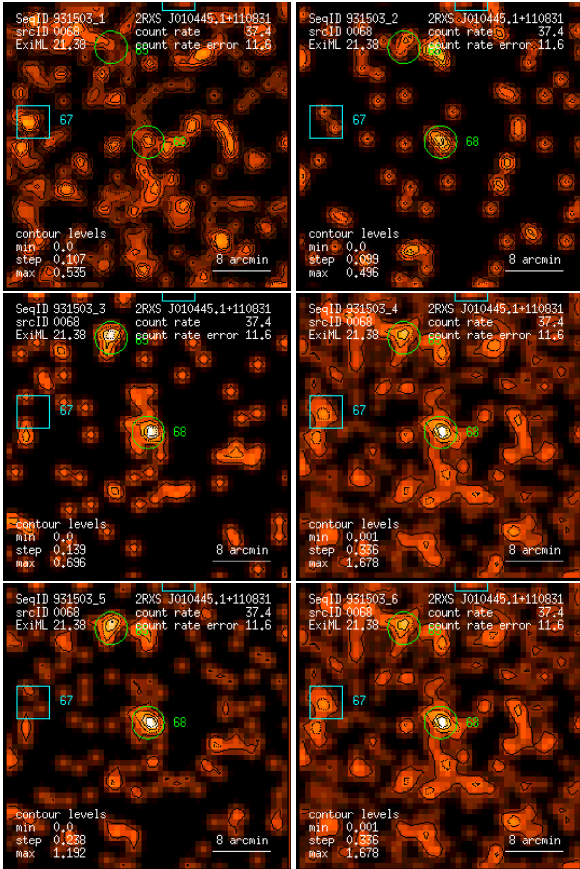
Figure 68: RASS 931503: detection 0068: band rate images, Gaussian filter: (1) PSPC channels 11 – 41, (2) 52 – 90, (3) 91 – 201, (4) 11 – 235, (5) 52 – 201, (6) 11 – 201. Broad band rates in counts/ks. Band rate contour levels in counts/ks/arcmin 2 .
