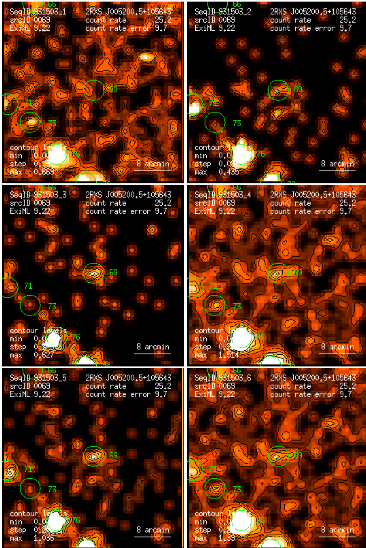
Figure 69: RASS 931503: detection 0069: band rate images, Gaussian filter: (1) PSPC channels 11 – 41, (2) 52 – 90, (3) 91 – 201, (4) 11 – 235, (5) 52 – 201, (6) 11 – 201. Broad band rates in counts/ks. Band rate contour levels in counts/ks/arcmin 2 .
