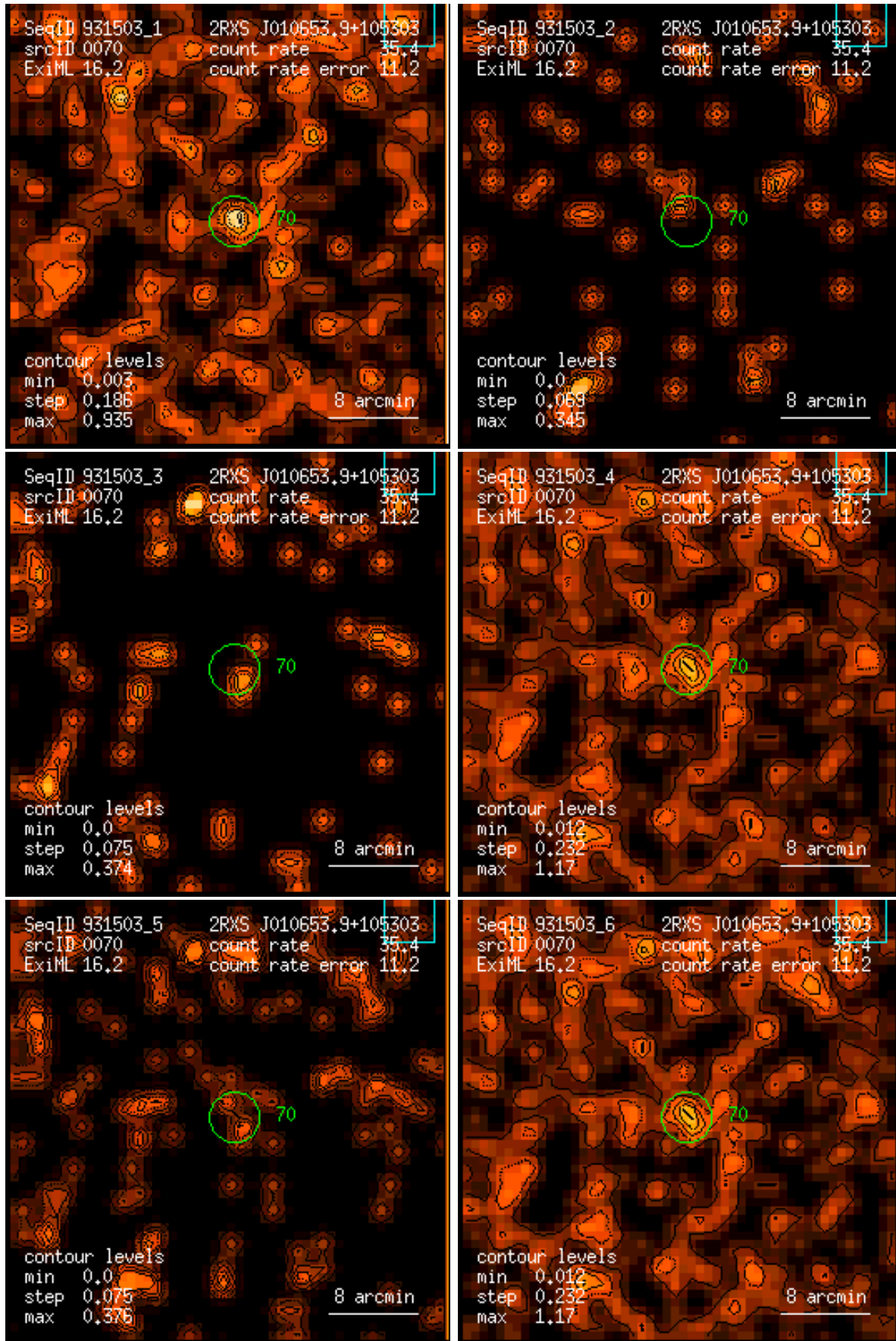
Figure 70: RASS 931503: detection 0070: band rate images, Gaussian filter: (1) PSPC channels 11 – 41, (2) 52 – 90, (3) 91 – 201, (4) 11 – 235, (5) 52 – 201, (6) 11 – 201. Broad band rates in counts/ks. Band rate contour levels in counts/ks/arcmin 2 .
