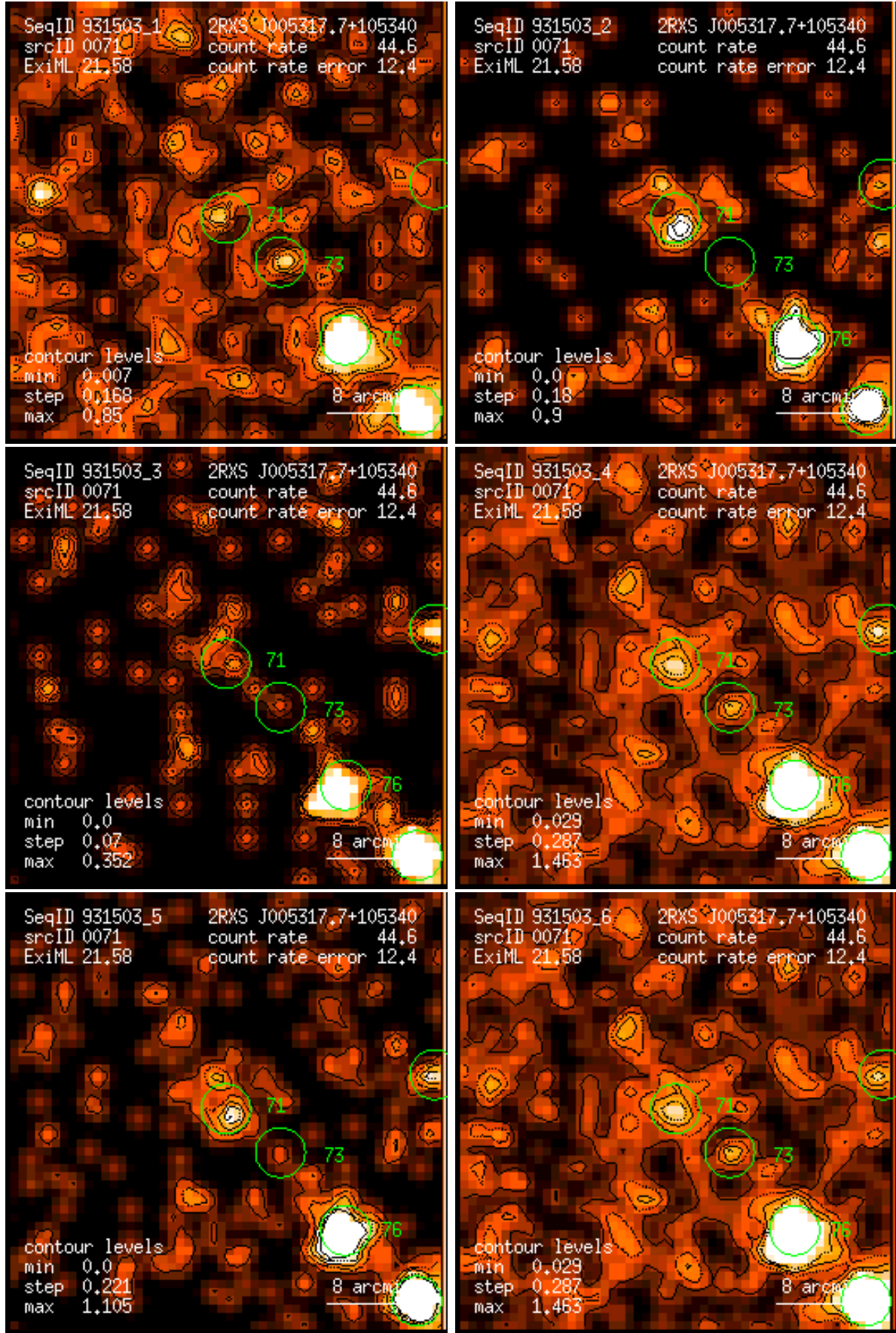
Figure 71: RASS 931503: detection 0071: band rate images, Gaussian filter: (1) PSPC channels 11 – 41, (2) 52 – 90, (3) 91 – 201, (4) 11 – 235, (5) 52 – 201, (6) 11 – 201. Broad band rates in counts/ks. Band rate contour levels in counts/ks/arcmin 2 .
