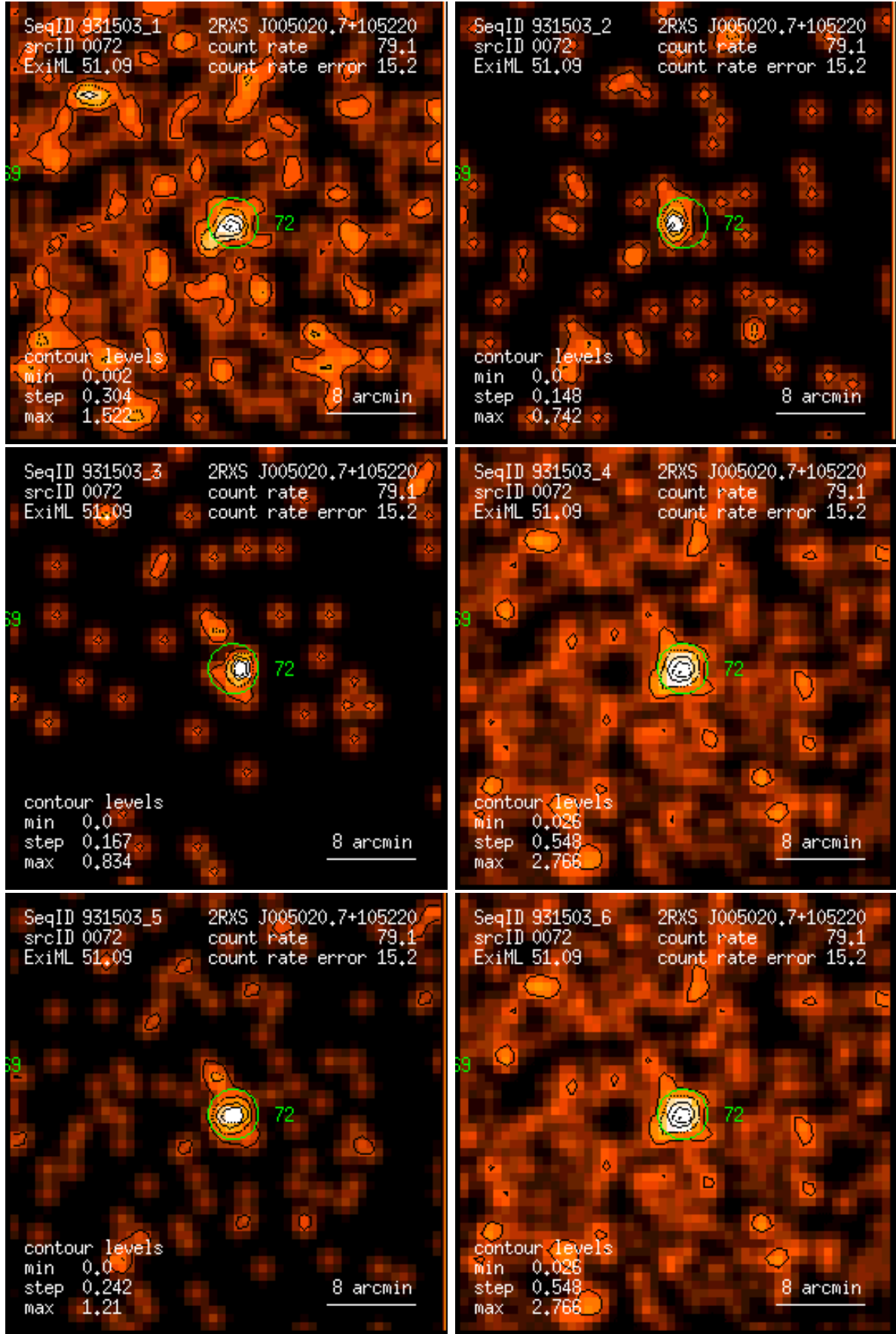
Figure 72: RASS 931503: detection 0072: band rate images, Gaussian filter: (1) PSPC channels 11 – 41, (2) 52 – 90, (3) 91 – 201, (4) 11 – 235, (5) 52 – 201, (6) 11 – 201. Broad band rates in counts/ks. Band rate contour levels in counts/ks/arcmin 2 .
