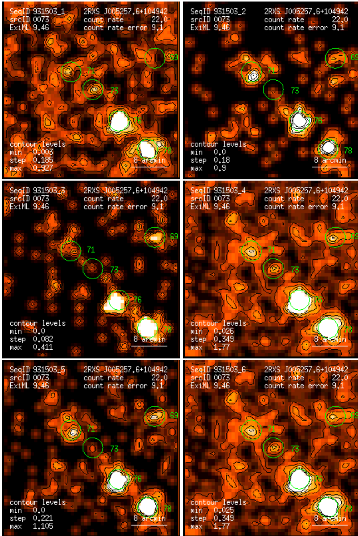
Figure 73: RASS 931503: detection 0073: band rate images, Gaussian filter: (1) PSPC channels 11 – 41, (2) 52 – 90, (3) 91 – 201, (4) 11 – 235, (5) 52 – 201, (6) 11 – 201. Broad band rates in counts/ks. Band rate contour levels in counts/ks/arcmin 2 .
