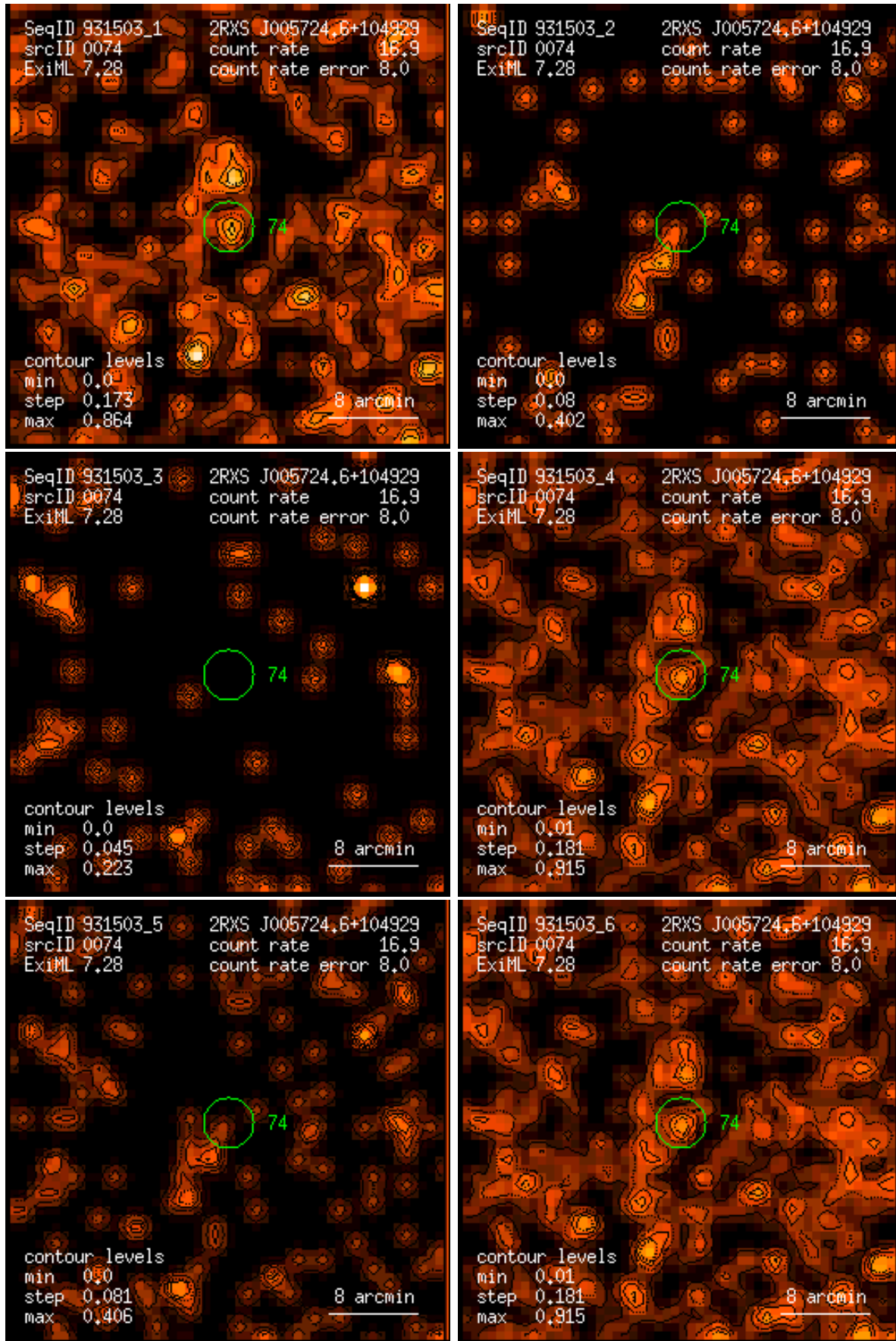
Figure 74: RASS 931503: detection 0074: band rate images, Gaussian filter: (1) PSPC channels 11 – 41, (2) 52 – 90, (3) 91 – 201, (4) 11 – 235, (5) 52 – 201, (6) 11 – 201. Broad band rates in counts/ks. Band rate contour levels in counts/ks/arcmin 2 .
