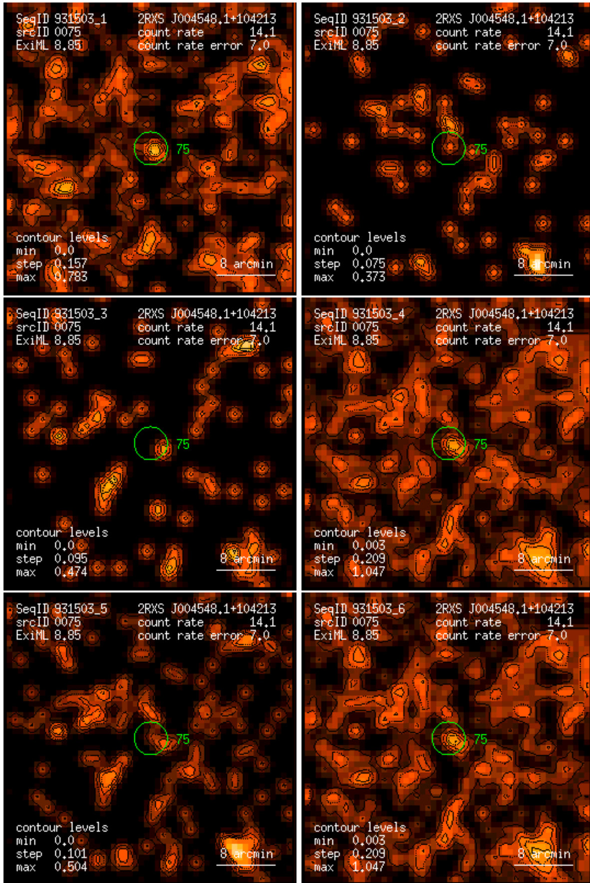
Figure 75: RASS 931503: detection 0075: band rate images, Gaussian filter: (1) PSPC channels 11 – 41, (2) 52 – 90, (3) 91 – 201, (4) 11 – 235, (5) 52 – 201, (6) 11 – 201. Broad band rates in counts/ks. Band rate contour levels in counts/ks/arcmin 2 .
