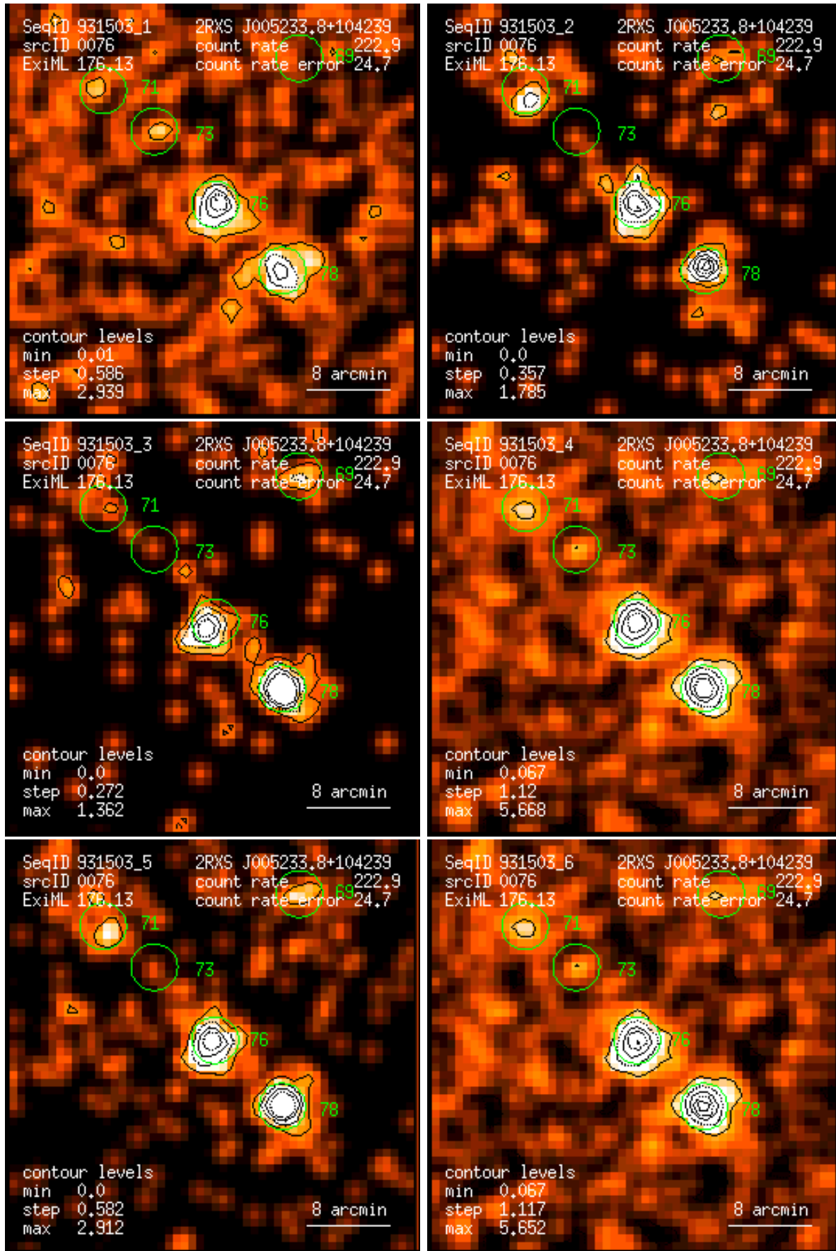
Figure 76: RASS 931503: detection 0076: band rate images, Gaussian filter: (1) PSPC channels 11 – 41, (2) 52 – 90, (3) 91 – 201, (4) 11 – 235, (5) 52 – 201, (6) 11 – 201. Broad band rates in counts/ks. Band rate contour levels in counts/ks/arcmin 2 .
