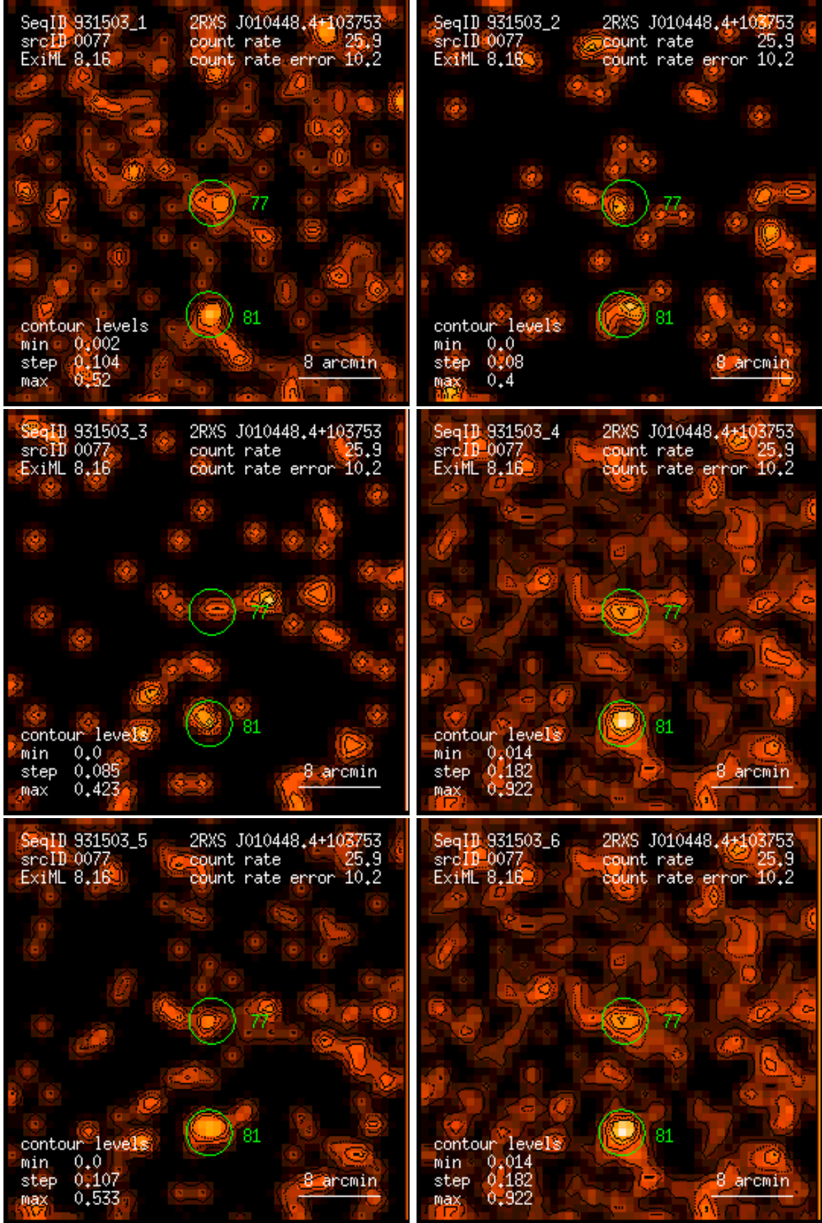
Figure 77: RASS 931503: detection 0077: band rate images, Gaussian filter: (1) PSPC channels 11 – 41, (2) 52 – 90, (3) 91 – 201, (4) 11 – 235, (5) 52 – 201, (6) 11 – 201. Broad band rates in counts/ks. Band rate contour levels in counts/ks/arcmin 2 .
