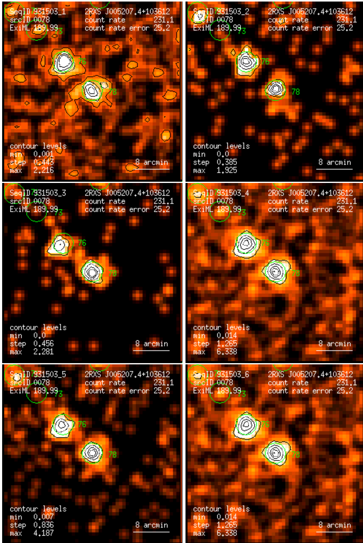
Figure 78: RASS 931503: detection 0078: band rate images, Gaussian filter: (1) PSPC channels 11 – 41, (2) 52 – 90, (3) 91 – 201, (4) 11 – 235, (5) 52 – 201, (6) 11 – 201. Broad band rates in counts/ks. Band rate contour levels in counts/ks/arcmin 2 .
