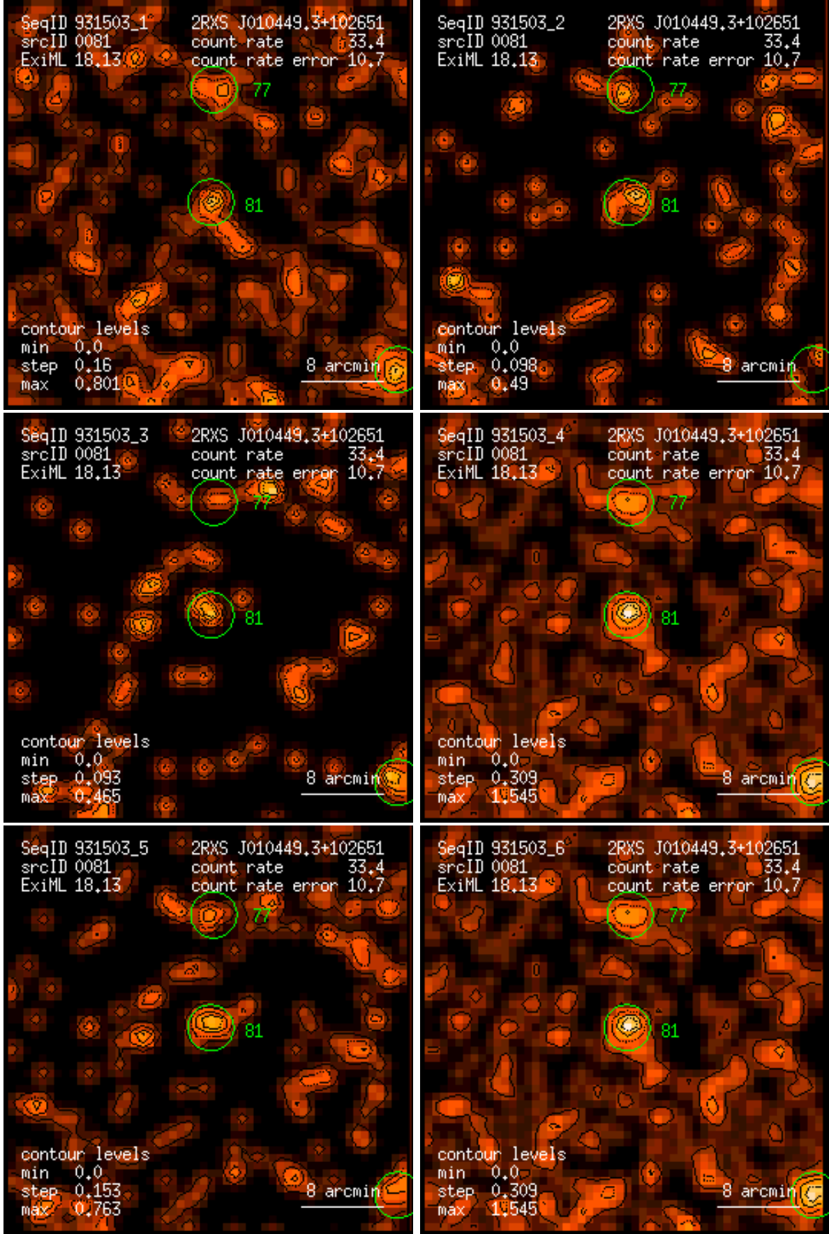
Figure 81: RASS 931503: detection 0081: band rate images, Gaussian filter: (1) PSPC channels 11 – 41, (2) 52 – 90, (3) 91 – 201, (4) 11 – 235, (5) 52 – 201, (6) 11 – 201. Broad band rates in counts/ks. Band rate contour levels in counts/ks/arcmin 2 .
