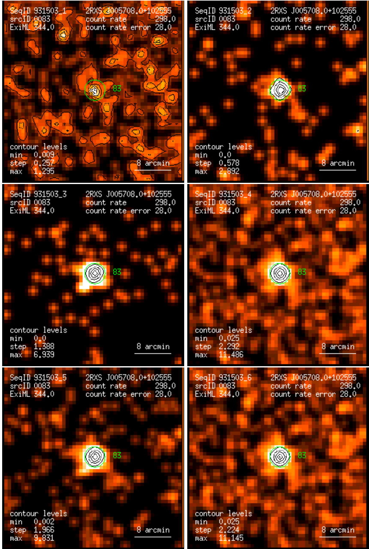
Figure 83: RASS 931503: detection 0083: band rate images, Gaussian filter: (1) PSPC channels 11 – 41, (2) 52 – 90, (3) 91 – 201, (4) 11 – 235, (5) 52 – 201, (6) 11 – 201. Broad band rates in counts/ks. Band rate contour levels in counts/ks/arcmin 2 .
