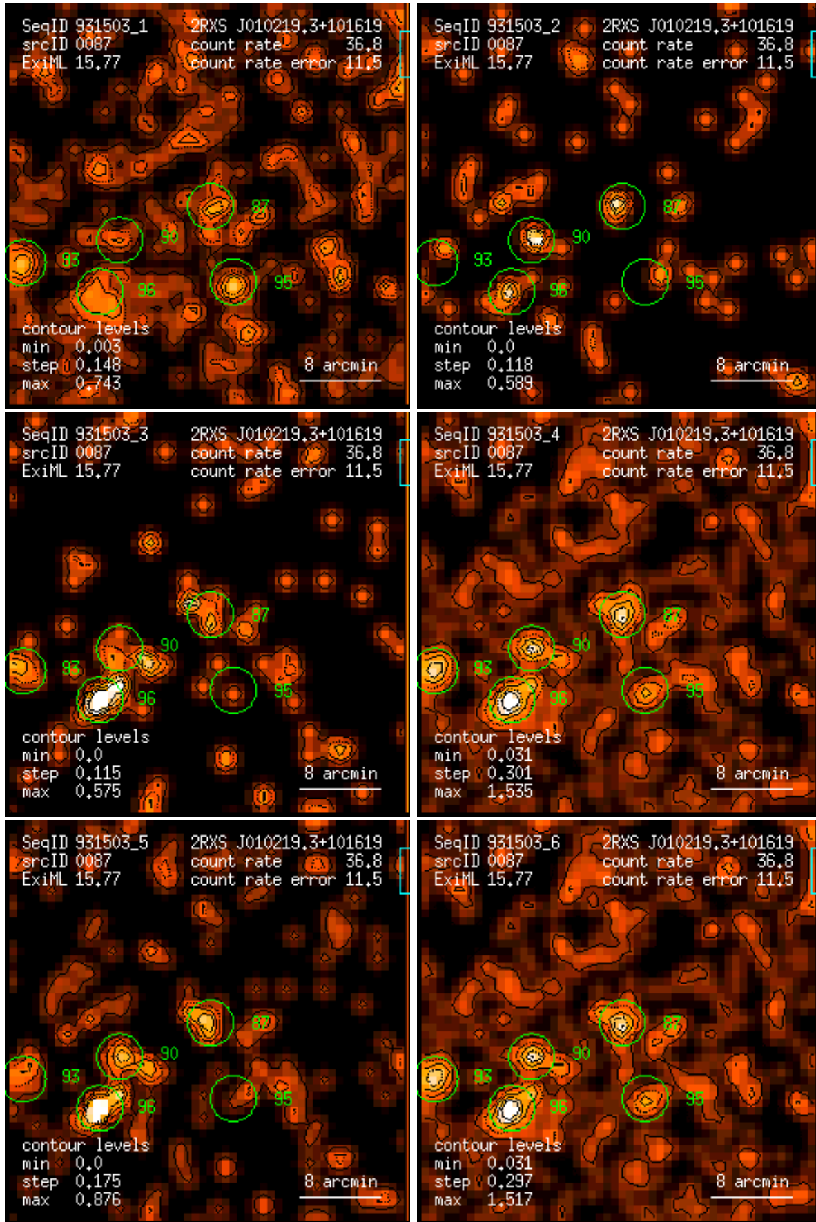
Figure 87: RASS 931503: detection 0087: band rate images, Gaussian filter: (1) PSPC channels 11 – 41, (2) 52 – 90, (3) 91 – 201, (4) 11 – 235, (5) 52 – 201, (6) 11 – 201. Broad band rates in counts/ks. Band rate contour levels in counts/ks/arcmin 2 .
