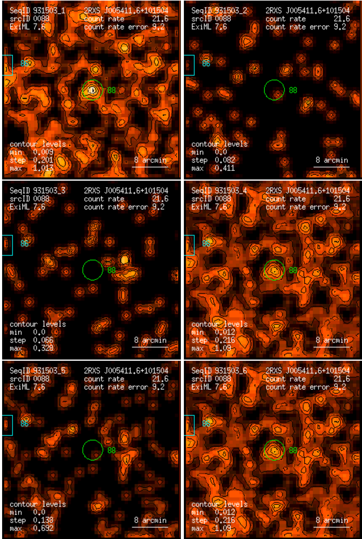
Figure 88: RASS 931503: detection 0088: band rate images, Gaussian filter: (1) PSPC channels 11 – 41, (2) 52 – 90, (3) 91 – 201, (4) 11 – 235, (5) 52 – 201, (6) 11 – 201. Broad band rates in counts/ks. Band rate contour levels in counts/ks/arcmin 2 .
