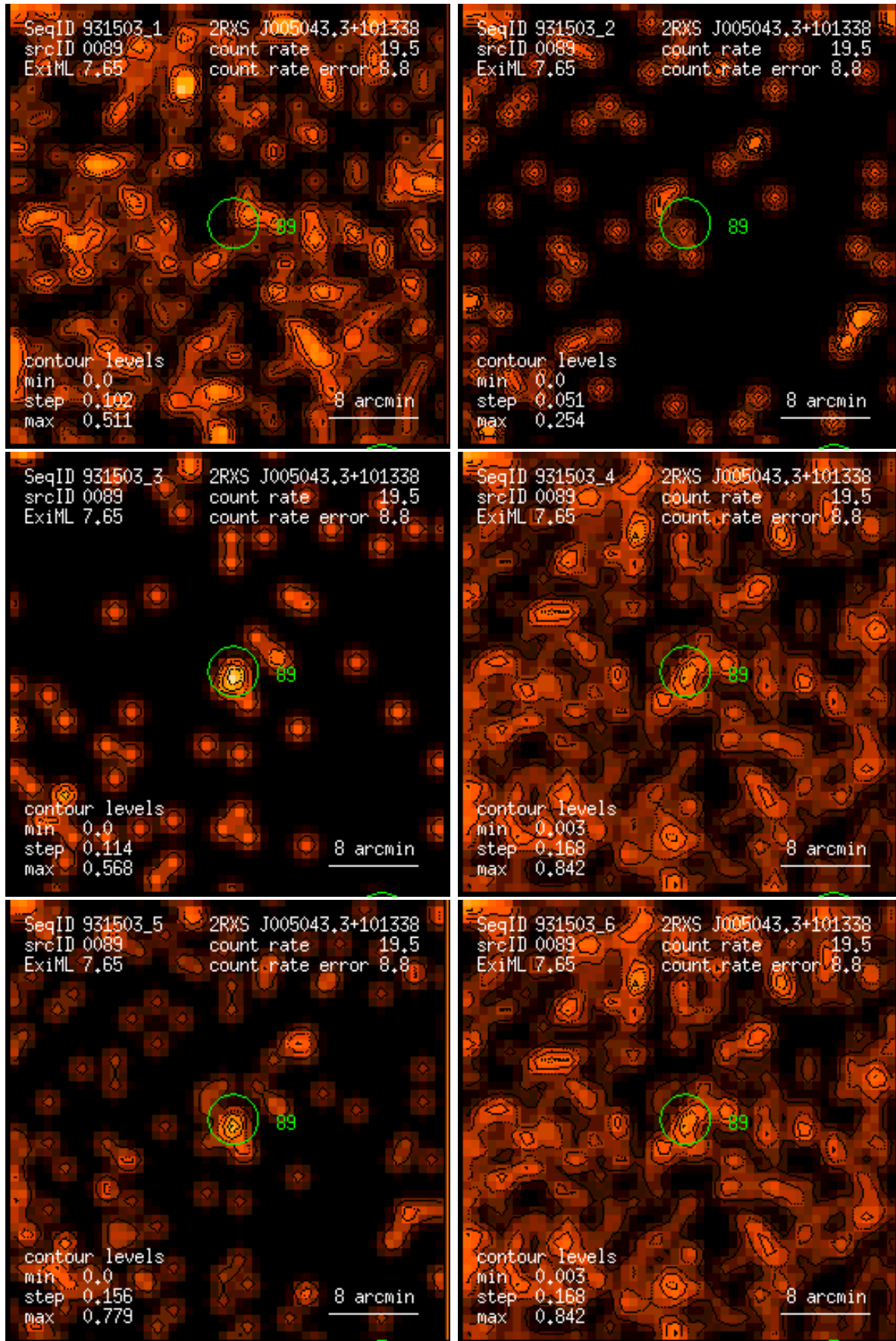
Figure 89: RASS 931503: detection 0089: band rate images, Gaussian filter: (1) PSPC channels 11 – 41, (2) 52 – 90, (3) 91 – 201, (4) 11 – 235, (5) 52 – 201, (6) 11 – 201. Broad band rates in counts/ks. Band rate contour levels in counts/ks/arcmin 2 .
