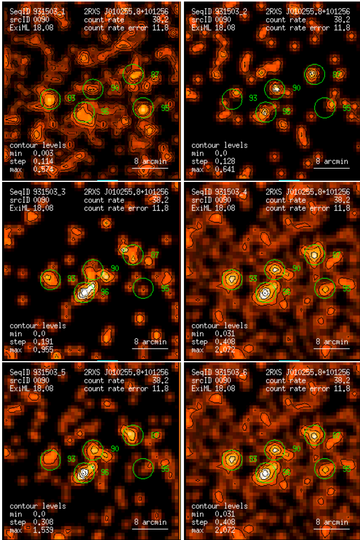
Figure 90: RASS 931503: detection 0090: band rate images, Gaussian filter: (1) PSPC channels 11 – 41, (2) 52 – 90, (3) 91 – 201, (4) 11 – 235, (5) 52 – 201, (6) 11 – 201. Broad band rates in counts/ks. Band rate contour levels in counts/ks/arcmin 2 .
