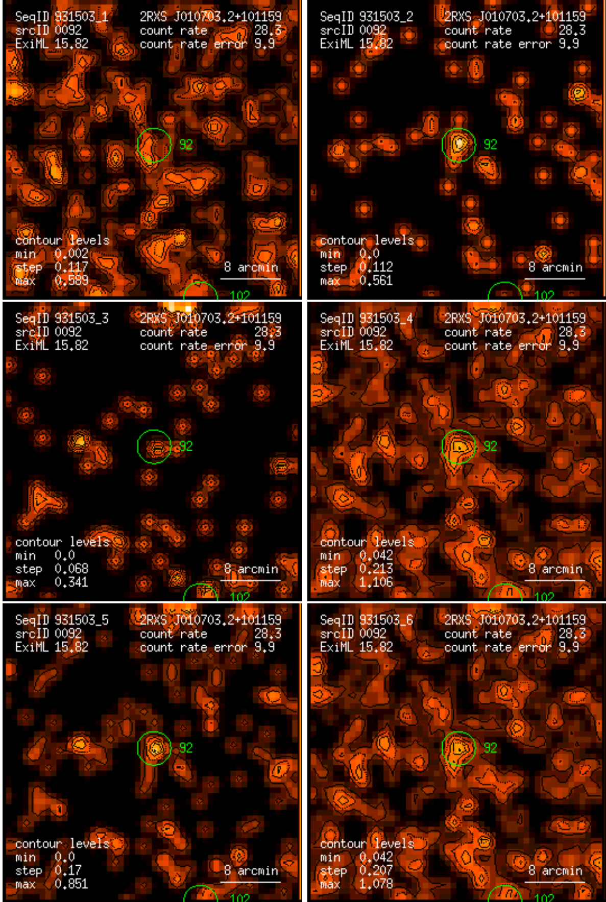
Figure 92: RASS 931503: detection 0092: band rate images, Gaussian filter: (1) PSPC channels 11 – 41, (2) 52 – 90, (3) 91 – 201, (4) 11 – 235, (5) 52 – 201, (6) 11 – 201. Broad band rates in counts/ks. Band rate contour levels in counts/ks/arcmin 2 .
