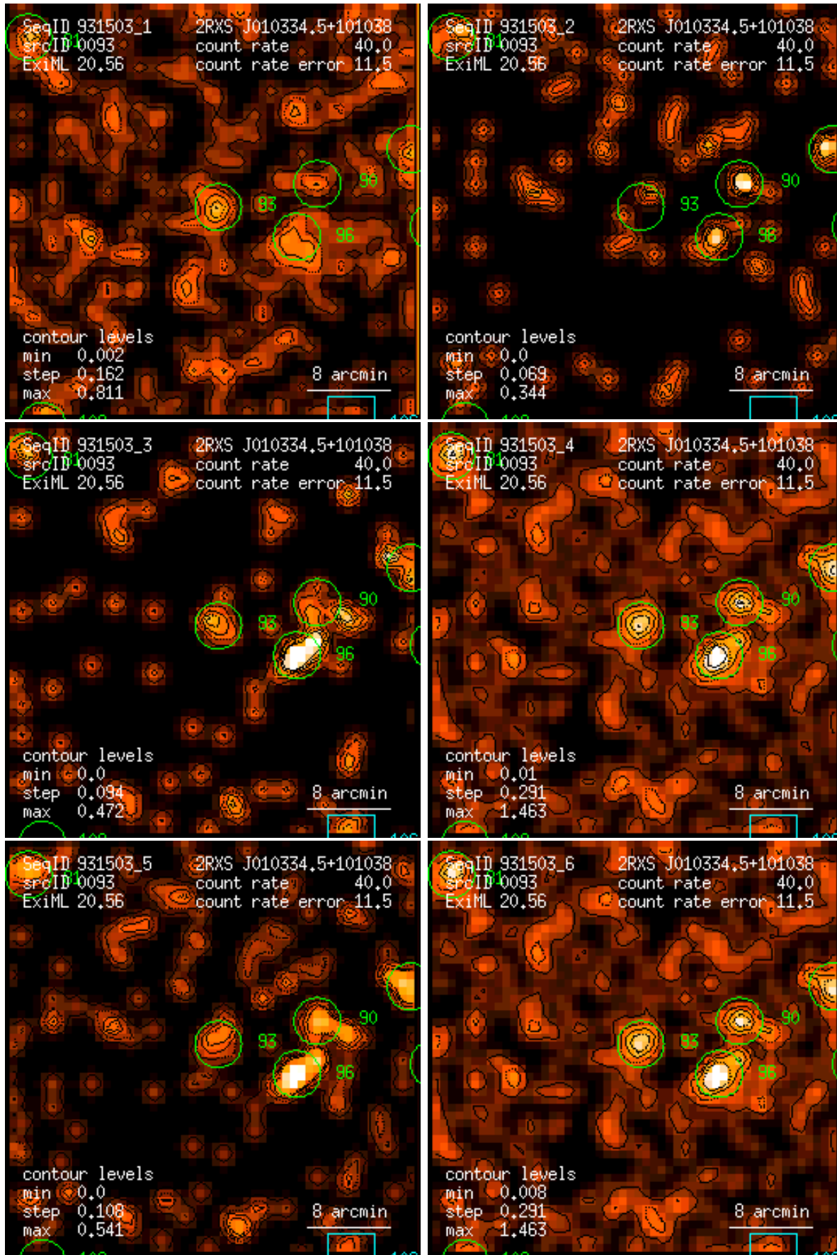
Figure 93: RASS 931503: detection 0093: band rate images, Gaussian filter: (1) PSPC channels 11 – 41, (2) 52 – 90, (3) 91 – 201, (4) 11 – 235, (5) 52 – 201, (6) 11 – 201. Broad band rates in counts/ks. Band rate contour levels in counts/ks/arcmin 2 .
