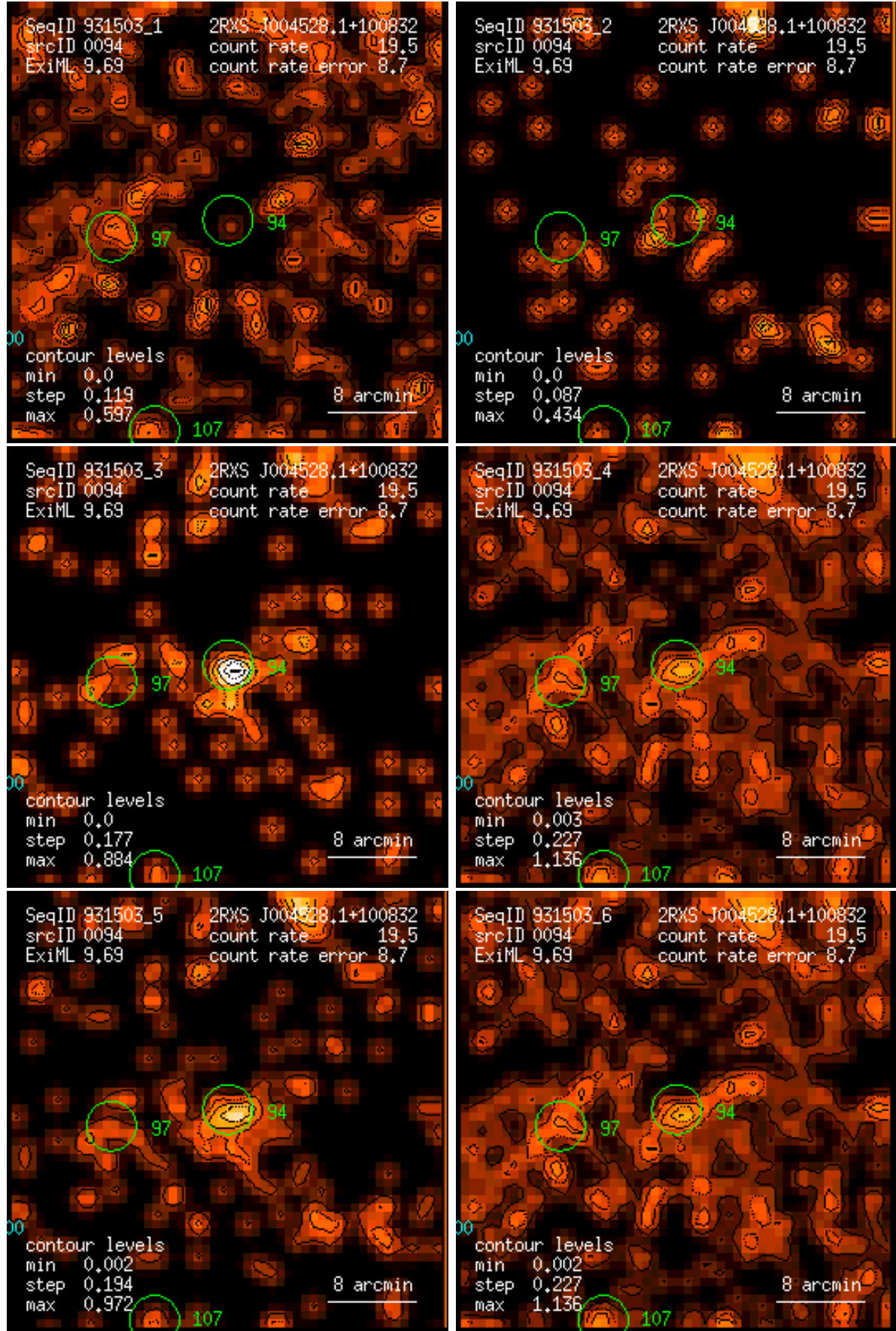
Figure 94: RASS 931503: detection 0094: band rate images, Gaussian filter: (1) PSPC channels 11 – 41, (2) 52 – 90, (3) 91 – 201, (4) 11 – 235, (5) 52 – 201, (6) 11 – 201. Broad band rates in counts/ks. Band rate contour levels in counts/ks/arcmin 2 .
