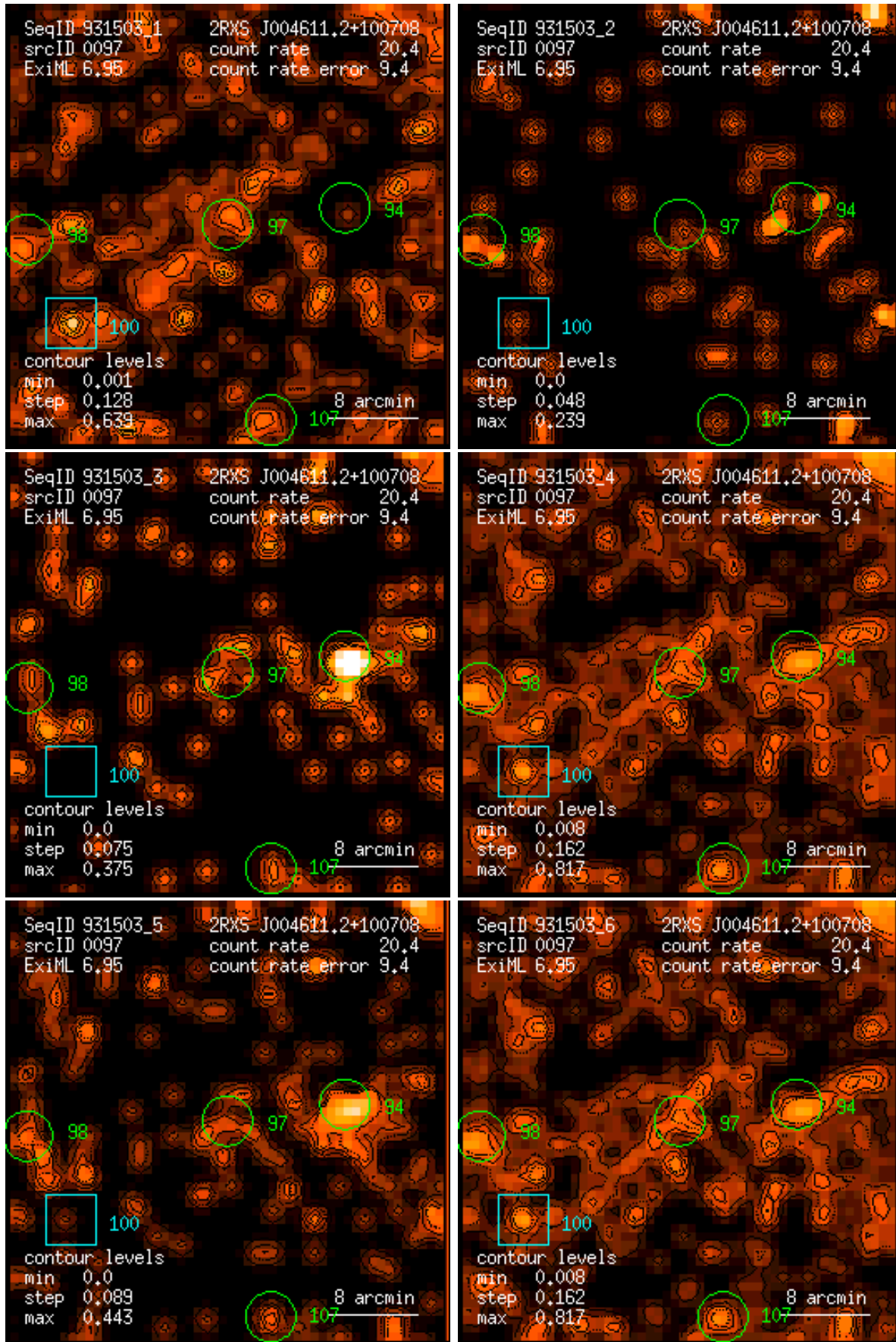
Figure 97: RASS 931503: detection 0097: band rate images, Gaussian filter: (1) PSPC channels 11 – 41, (2) 52 – 90, (3) 91 – 201, (4) 11 – 235, (5) 52 – 201, (6) 11 – 201. Broad band rates in counts/ks. Band rate contour levels in counts/ks/arcmin 2 .
