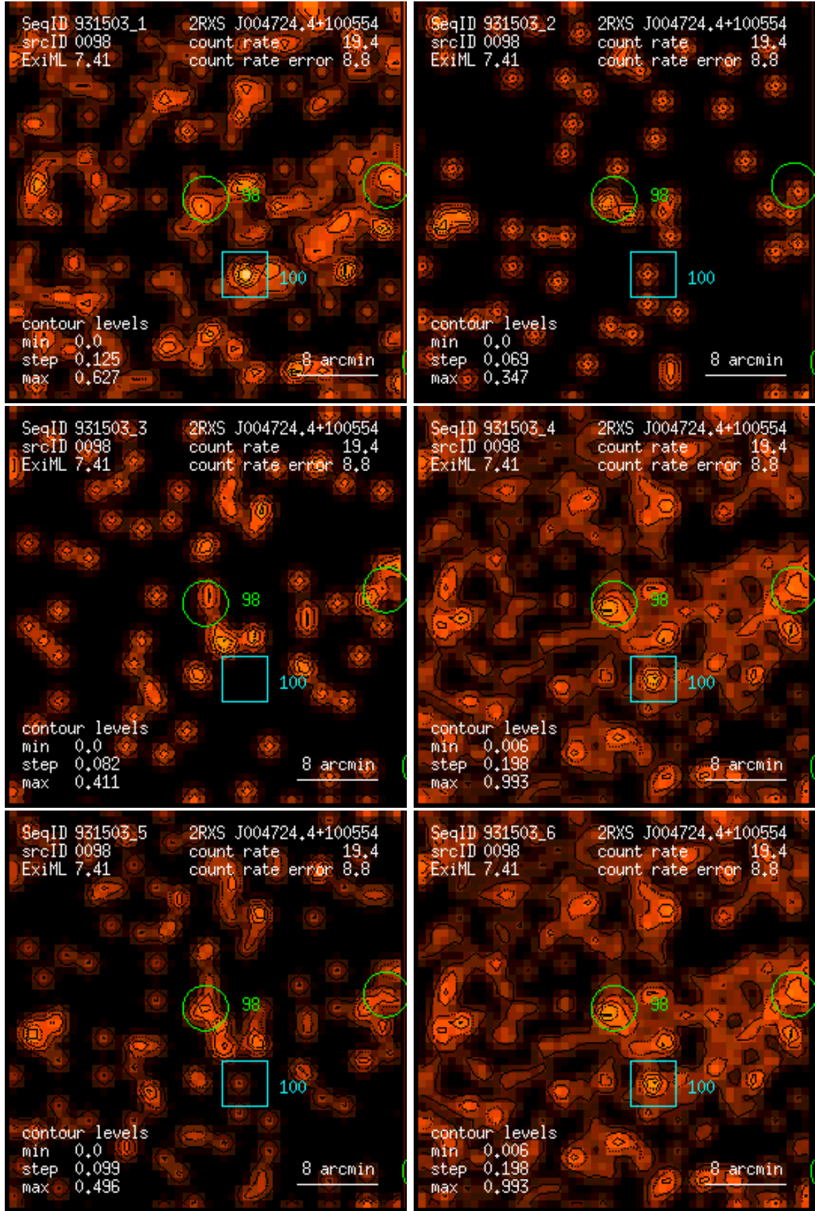
Figure 98: RASS 931503: detection 0098: band rate images, Gaussian filter: (1) PSPC channels 11 – 41, (2) 52 – 90, (3) 91 – 201, (4) 11 – 235, (5) 52 – 201, (6) 11 – 201. Broad band rates in counts/ks. Band rate contour levels in counts/ks/arcmin 2 .
