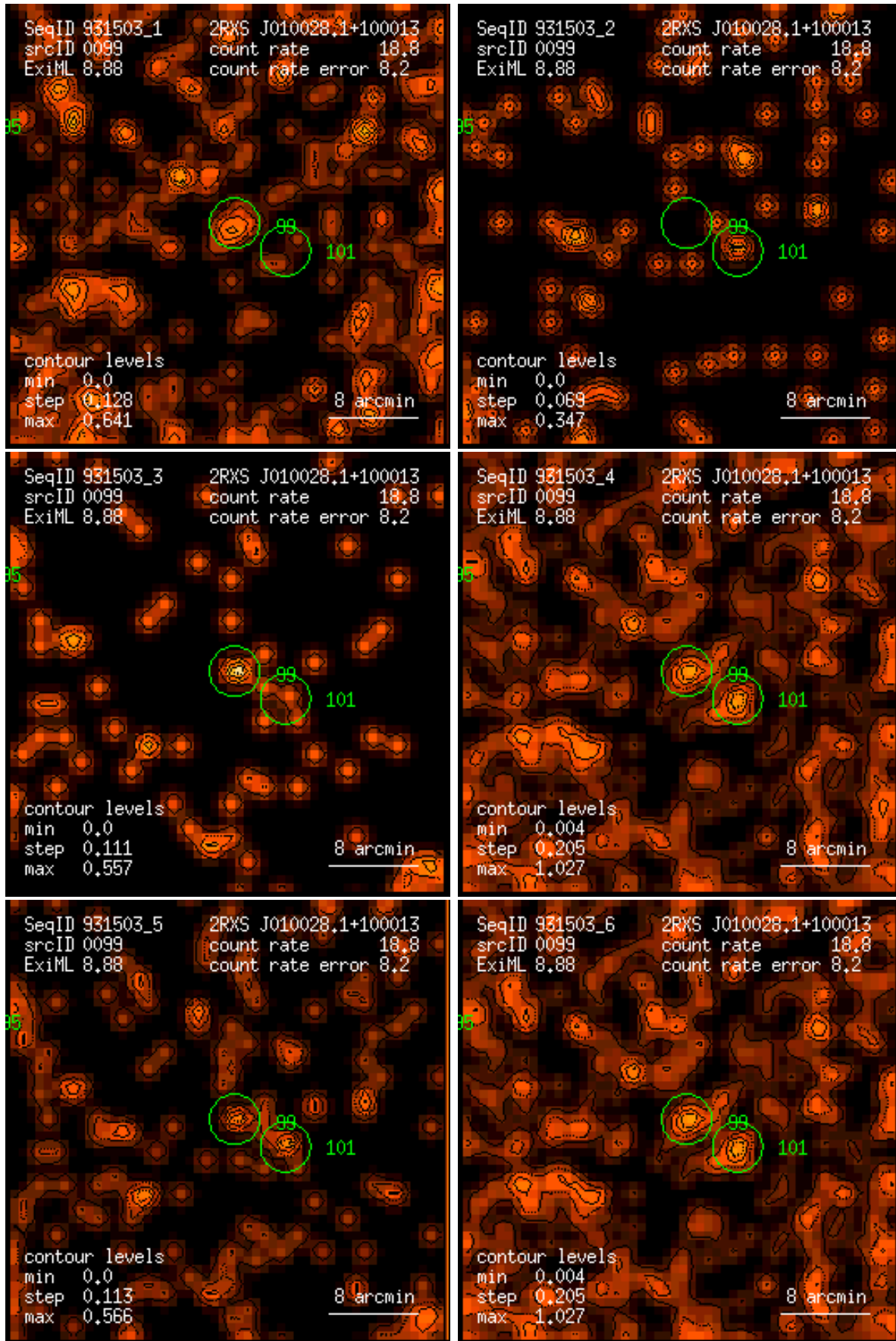
Figure 99: RASS 931503: detection 0099: band rate images, Gaussian filter: (1) PSPC channels 11 – 41, (2) 52 – 90, (3) 91 – 201, (4) 11 – 235, (5) 52 – 201, (6) 11 – 201. Broad band rates in counts/ks. Band rate contour levels in counts/ks/arcmin 2 .
