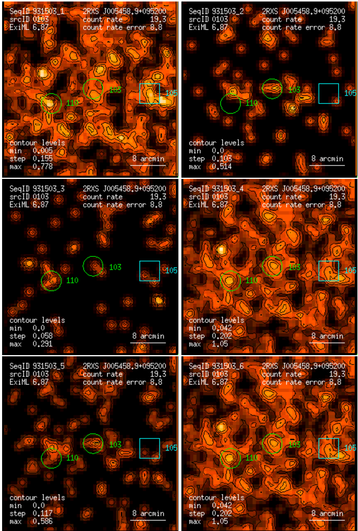
Figure 103: RASS 931503: detection 0103: band rate images, Gaussian filter: (1) PSPC channels 11 – 41, (2) 52 – 90, (3) 91 – 201, (4) 11 – 235, (5) 52 – 201, (6) 11 – 201. Broad band rates in counts/ks. Band rate contour levels in counts/ks/arcmin 2 .
