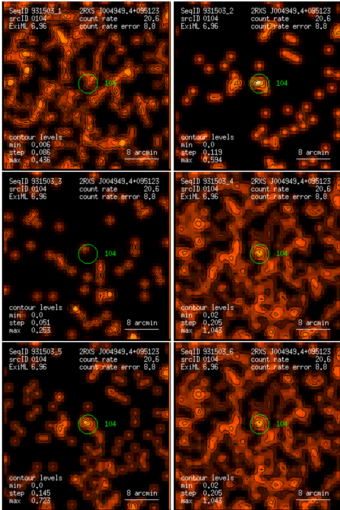
Figure 104: RASS 931503: detection 0104: band rate images, Gaussian filter: (1) PSPC channels 11 – 41, (2) 52 – 90, (3) 91 – 201, (4) 11 – 235, (5) 52 – 201, (6) 11 – 201. Broad band rates in counts/ks. Band rate contour levels in counts/ks/arcmin 2 .
