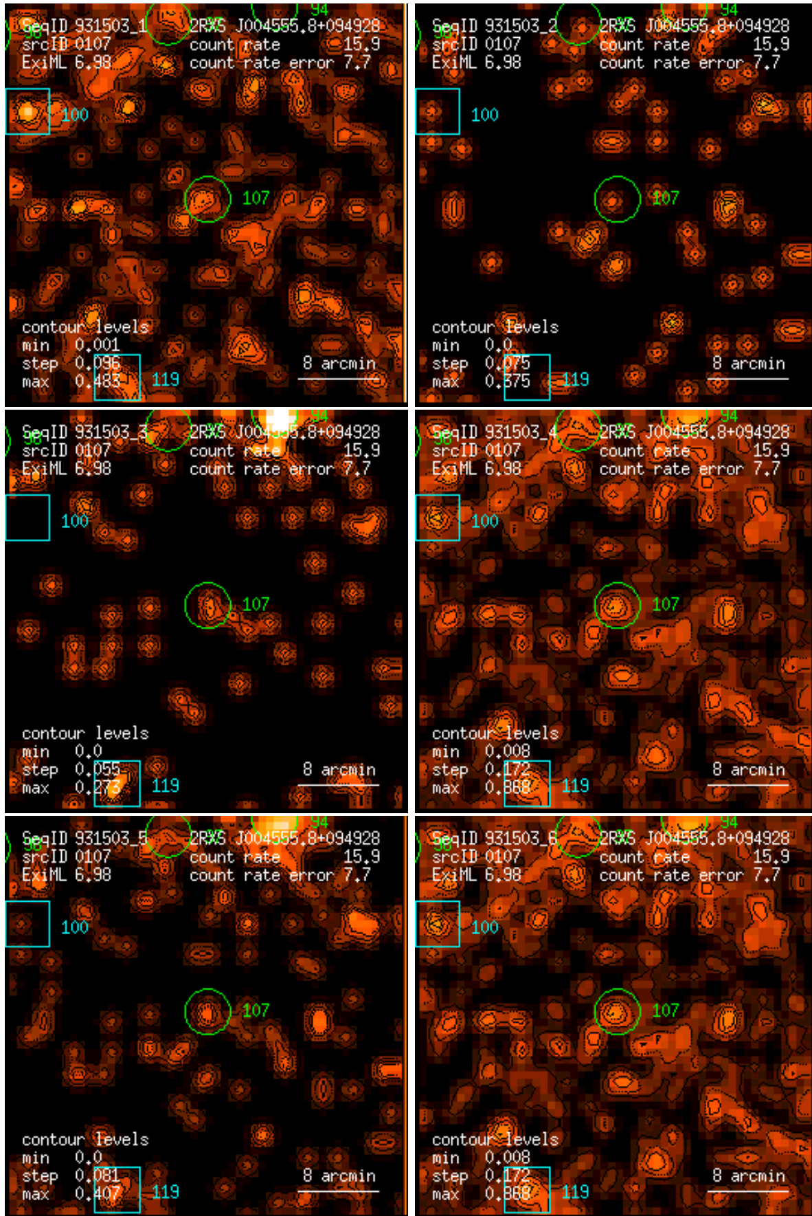
Figure 107: RASS 931503: detection 0107: band rate images, Gaussian filter: (1) PSPC channels 11 – 41, (2) 52 – 90, (3) 91 – 201, (4) 11 – 235, (5) 52 – 201, (6) 11 – 201. Broad band rates in counts/ks. Band rate contour levels in counts/ks/arcmin 2 .
